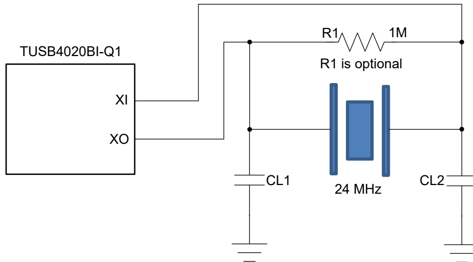
Figure 8-1. TUSB4020BI-Q1 Clock
