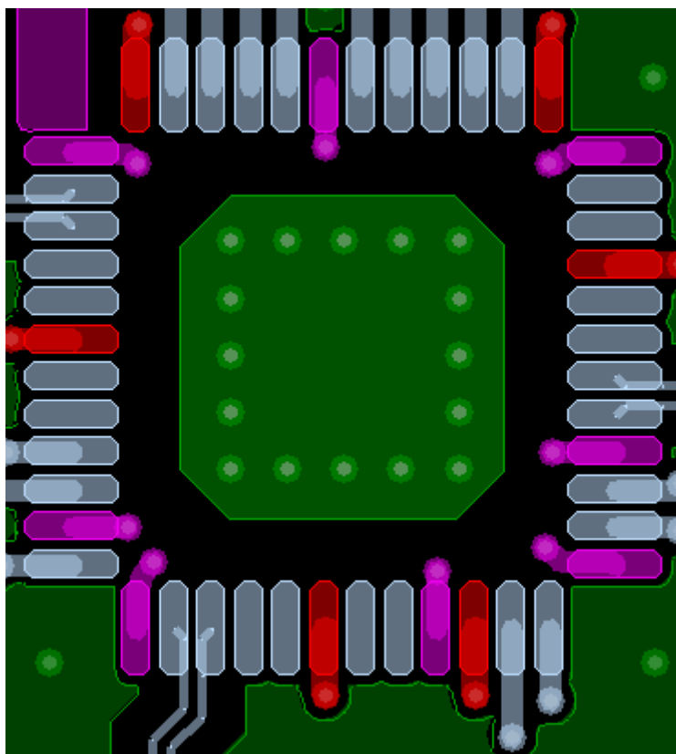
Figure 11-3. Thermal Pad
