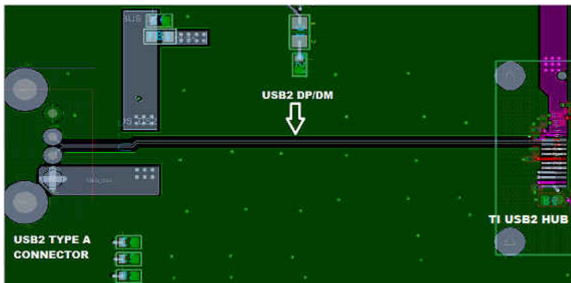
Figure 11-2. Downstream Port
