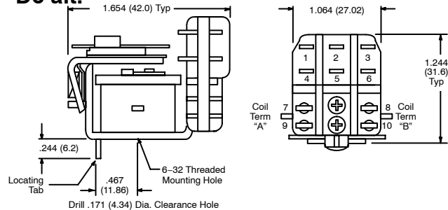
A (SPDT), 1 Form "C" B (DPDT), 2 Form "C" C (3PDT), 3 Form "C"
