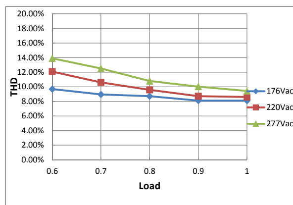
THD Curve
