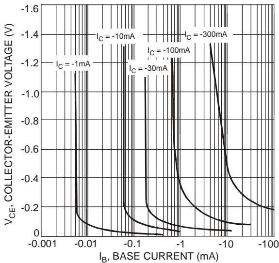
Fig. 5 Typical Collector Saturation Region
