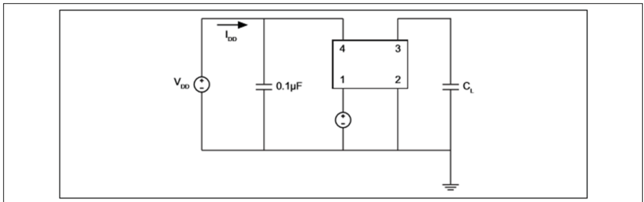
FIGURE 5-1: Test Circuit.
