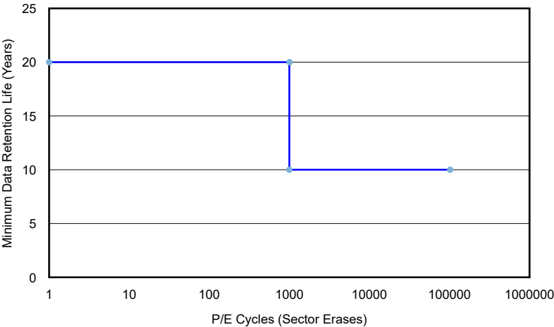
Figure 15. Data retention vs program/erase cycles
