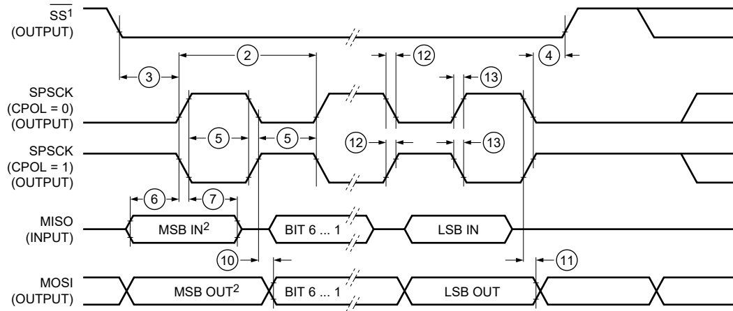
Figure 23. LPSPI Master Mode Timing (CPHA=0)
