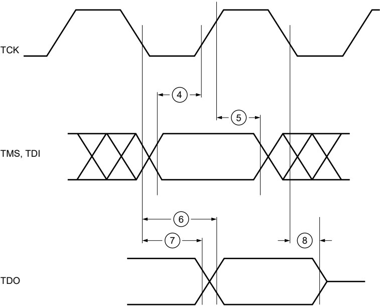
Figure 44. JTAG Test Access Port Timing
