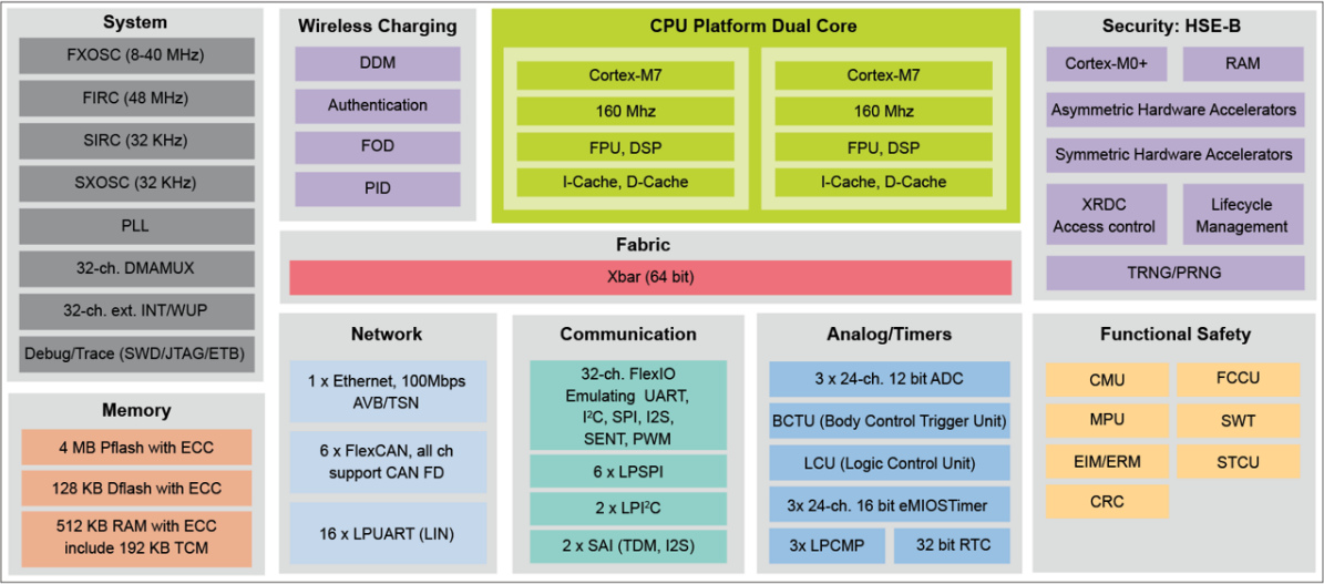
Figure 5. MWCT2D17S: ASIL B Dual Core 4MB General Purpose MCU
