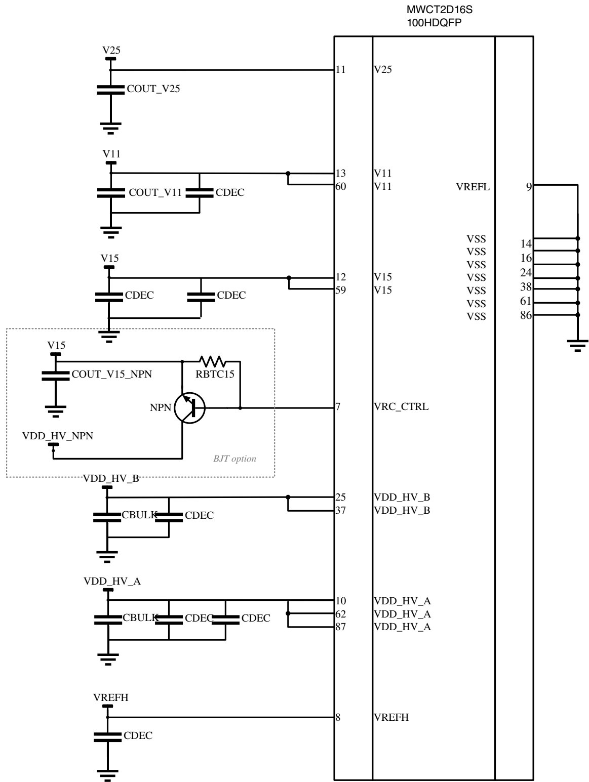
Figure 9. 100-pin HDQFP decoupling capacitor pinout diagram (MWCTD16S)
