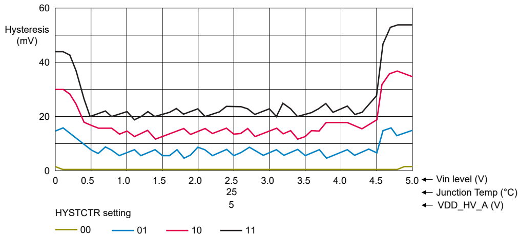
Figure 20. Typical Hysteresis vs Vin level (VDD_HV_A = 5 V, Low Speed Mode).png
