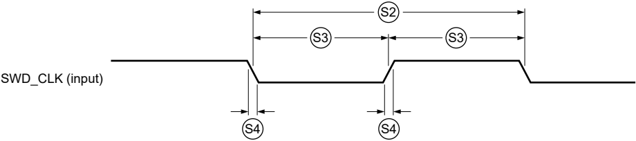
Figure 41. SWD Input Clock Timing
