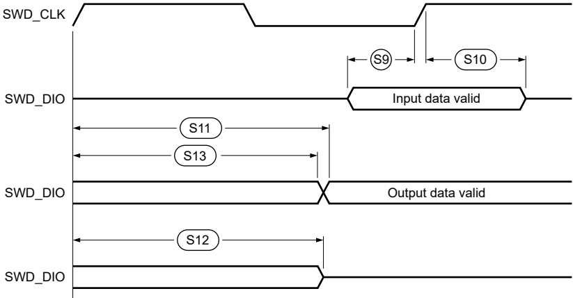
Figure 42. SWD Output Data Timing
