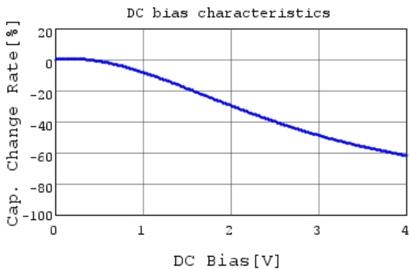
GRM32ER60G227ME05 C-DC bias capchange, 25.0C
