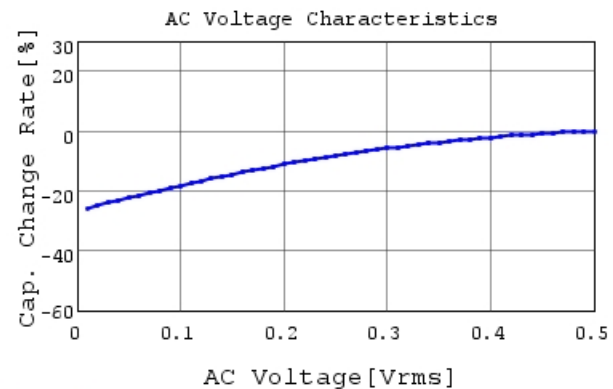
GRM32ER60G227ME05 C-AC Voltage capchange, D
