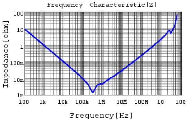
GRM32ER60G227ME05 |Z| DCOV, 25degC
