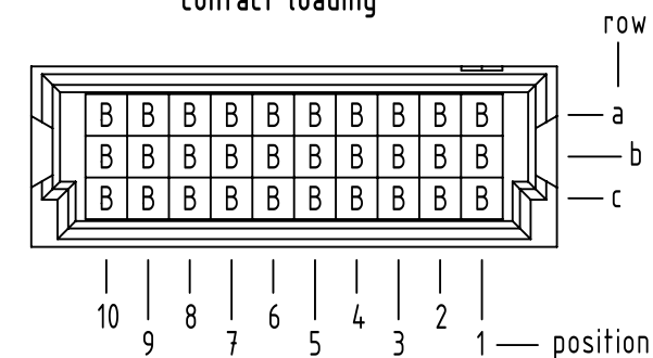
B (2:1) contact loading
