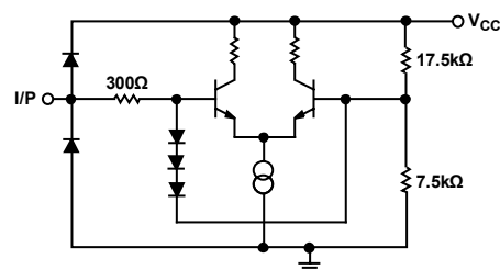
Figure 11. Equivalent I/P Input Circuit
