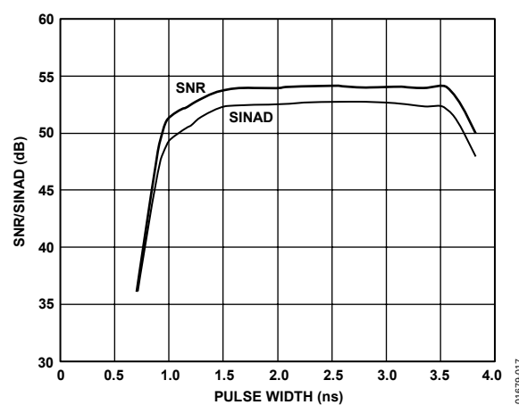
Figure 17. SNR/SINAD vs. Clock Positive Pulse Width ( f_s = 210 MSPS, A_{IN} = 70 MHz)
