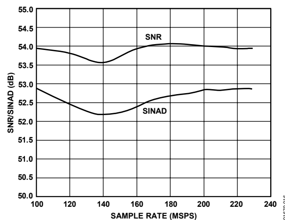
Figure 16. SNR/SINAD vs. Sample Rate; A_{IN} = 70 MHz
