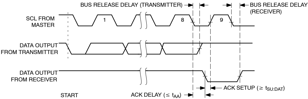
Figure 4. Acknowledge Timing
