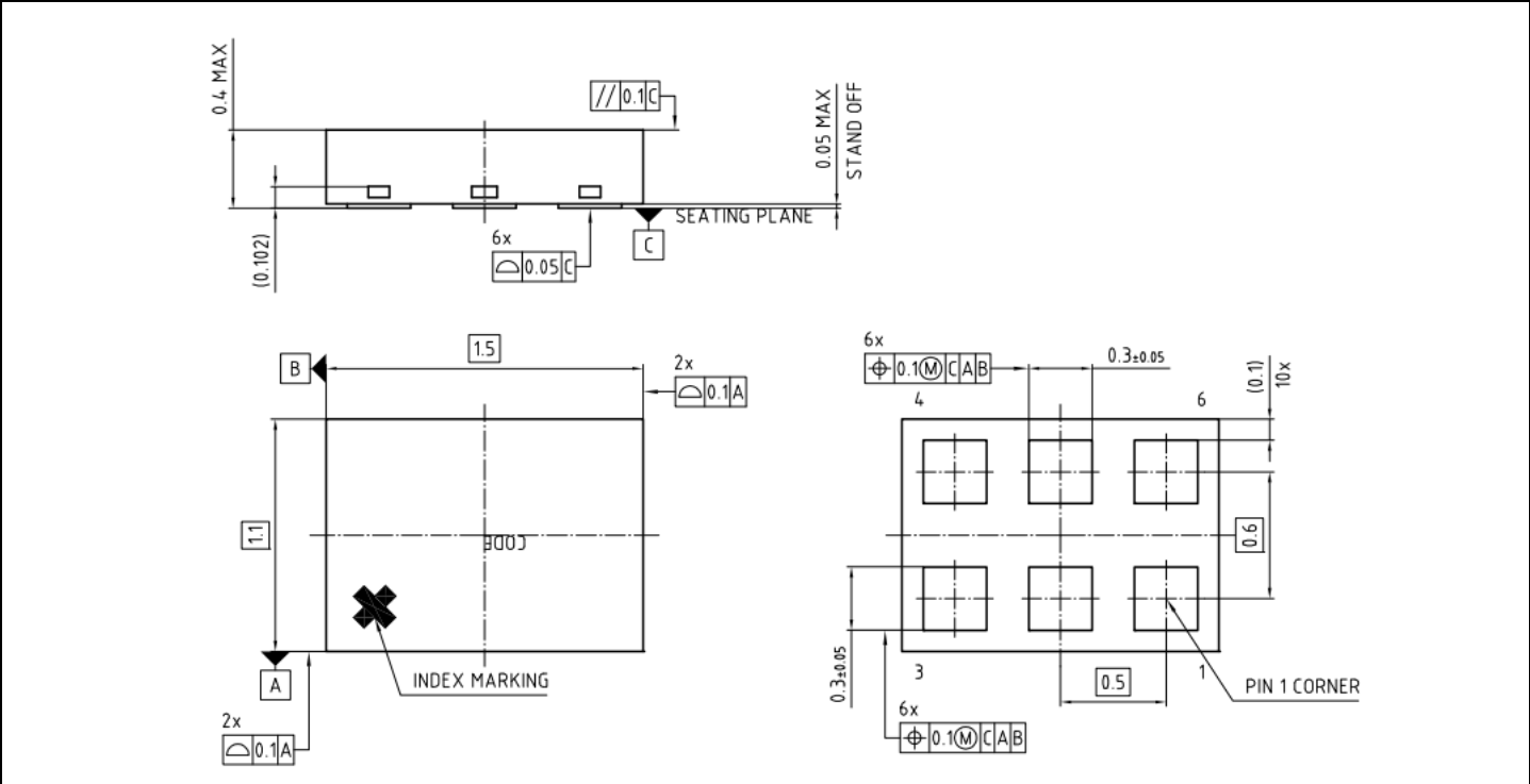
Figure 19 TSNP-6 outline
