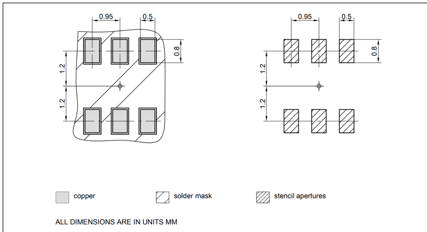
Figure 16 PG-SOT23-6 footprint
