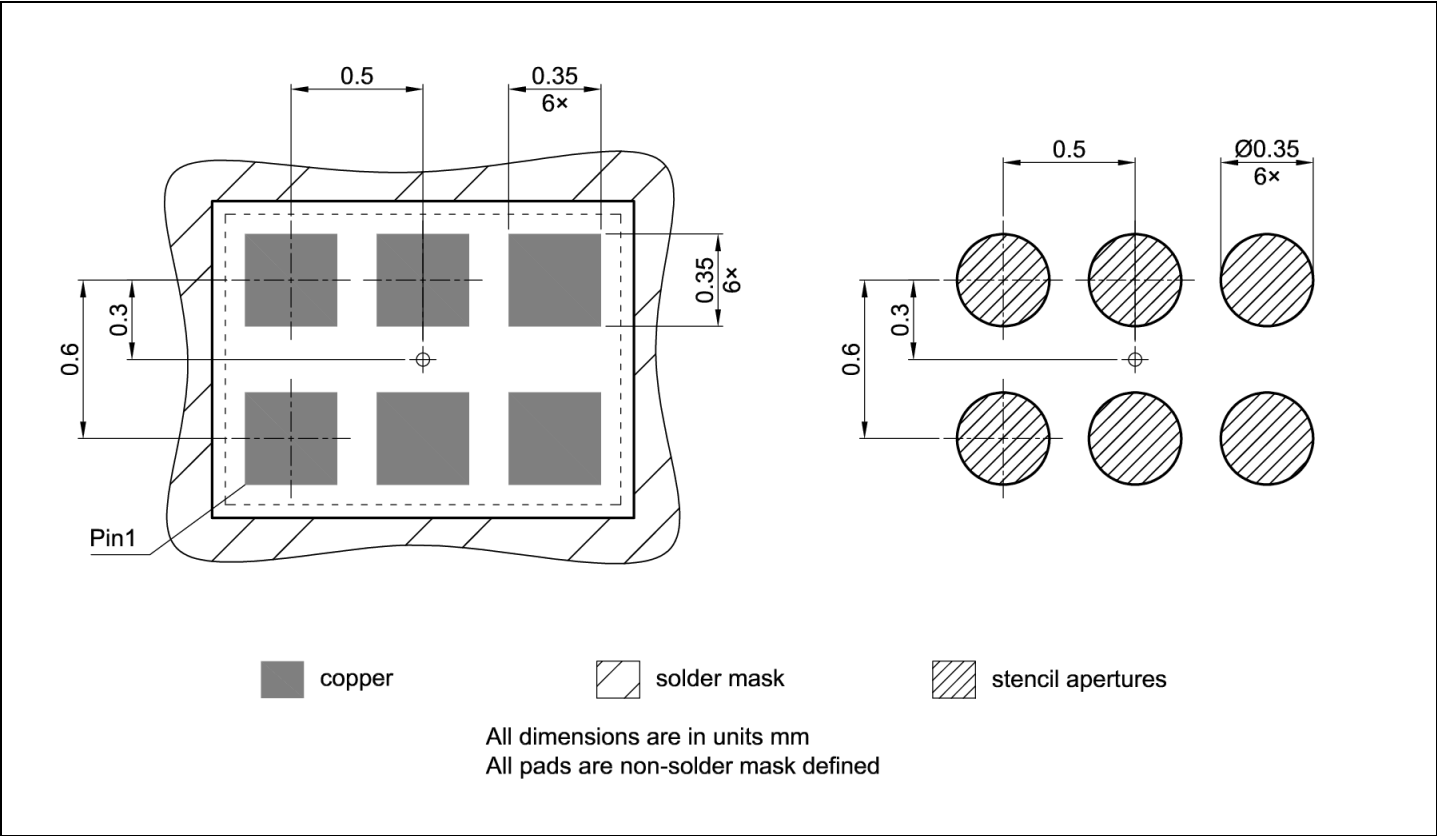
Figure 20 TSNP-6 footprint
