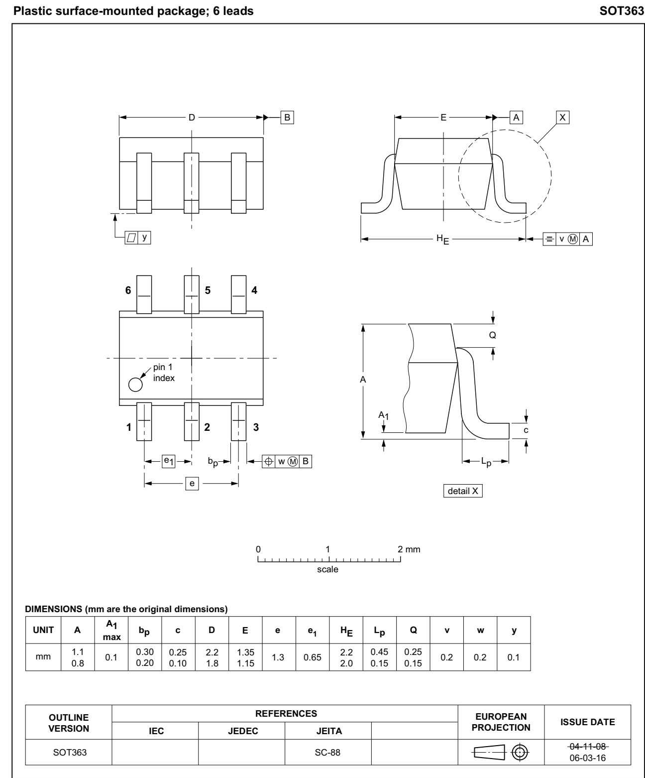
Fig 15. Package outline SOT363 (SC-88)
