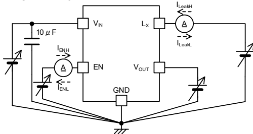
< Circuit No.5 >
