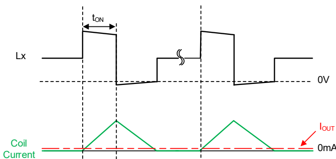
XC9286 series : Example of light load operation
