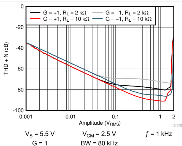
Figure 7-20. THD + N vs Amplitude
