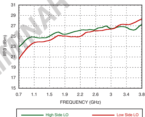
Figure 81. Input IP3 vs. High Side LO & Low Side LO @ VGATE=5V
