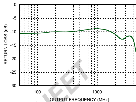
Figure 67. Auxiliary LO Single Ended Output Return Loss
