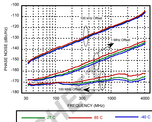
Figure 55. Auxiliary LO Output, Open Loop Phase Noise vs. Temperature
