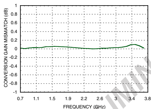
Figure 39. Low Side LO Conversion Gain Mismatch @ VGATE=5V [1]
