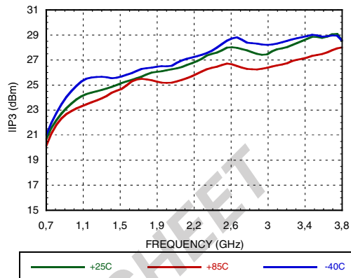
Figure 20. Low Side LO Input IP3 vs. Frequency @ VGATE=5V [2]
