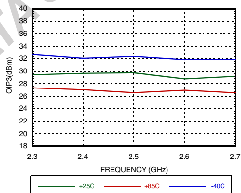
Figure 79. Conversion Gain, IIP3 and OIP3 for 2500MHz RF frequency bands. [1]
