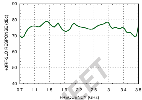
Figure 14. +3RF -3LO Response vs. Frequency over Temperature [1][2][3]
