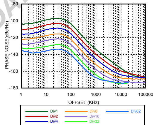
Figure 53. Auxiliary LO Output, Fractional Mode Closed Loop Phase Noise @ 3300 MHz with various divider ratios [2]
