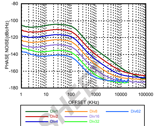
Figure 52. Auxiliary LO Output, Fractional Mode Closed Loop Phase Noise @4100 MHz with various divider ratios [1]
