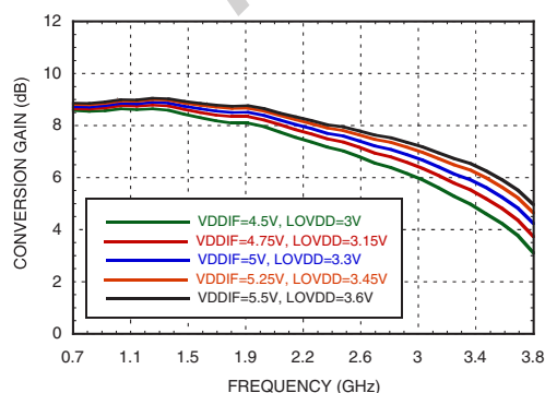
Figure 41. Low Side LO Conversion Gain vs. VGATE=Vdd [1]
