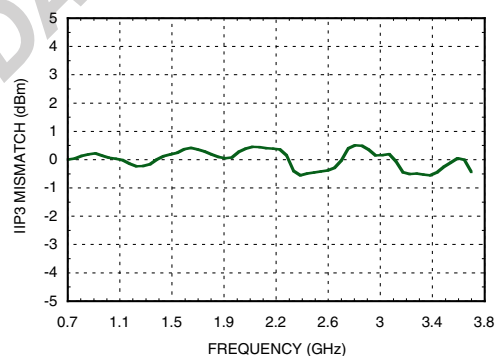
Figure 40. Low Side LO Input IP3 Mismatch @ VGATE=5V
