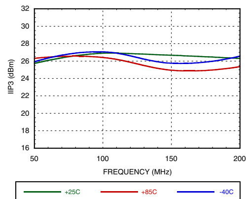
Figure 48. IIP3 vs. IF Frequency @ RF=2400 MHz, VGATE=5V
