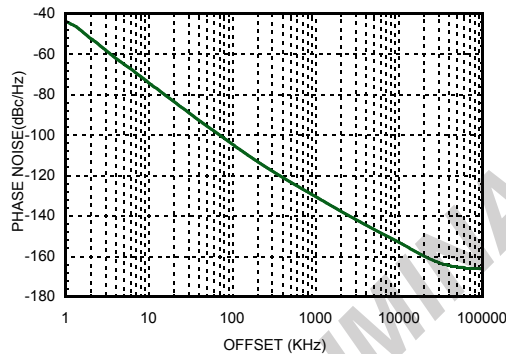
Figure 51. Auxiliary LO Output, Open Loop Phase Noise @ 4100 MHz
