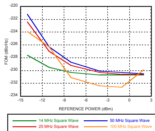
Figure 59. Reference Input Sensitivity, Square Wave, 50 \Omega [3]
