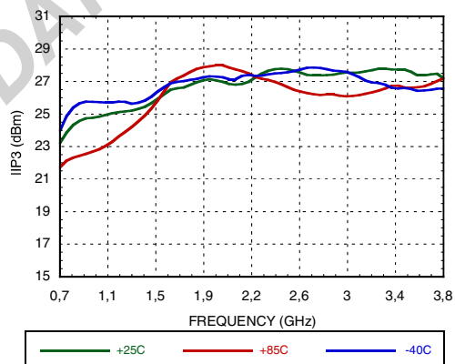
Figure 22. High Side LO Input IP3 vs. Frequency @ VGATE=5V [2]
