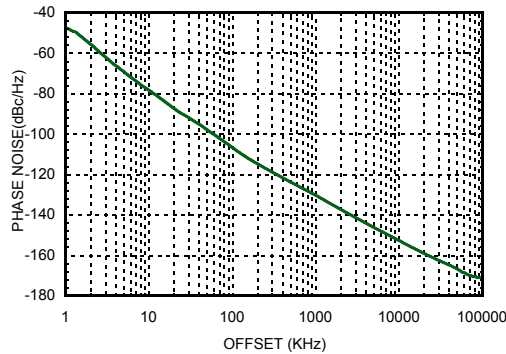
Figure 49. Auxiliary LO Output, Open Loop Phase Noise @ 3600 MHz
