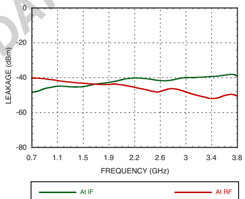
Figure 10. LO Leakage vs. Frequency [2][3]
