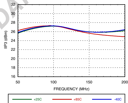
Figure 46. IIP3 vs. IF Frequency @ RF=1900 MHz, VGATE=5V
