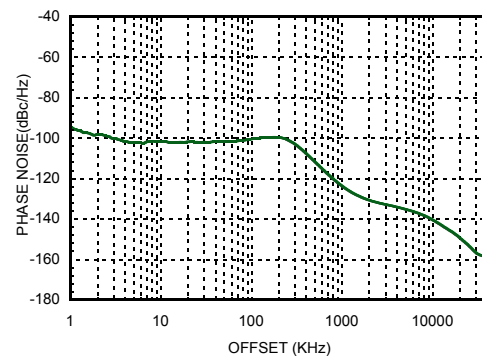
Figure 65. Closed Loop Phase Noise With External VCO HMC384LP4E @ 2200 MHz
