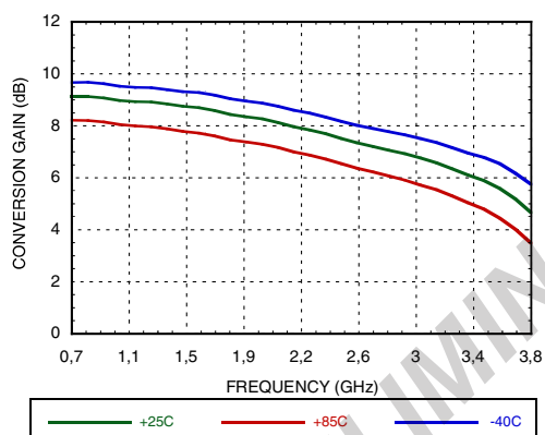
Figure 27. High Side LO Conversion Gain vs. Frequency @ VGATE=4.9V [1][2]
