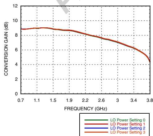
Figure 11. Low Side LO Conversion Gain vs. LO Drive [1][2]
