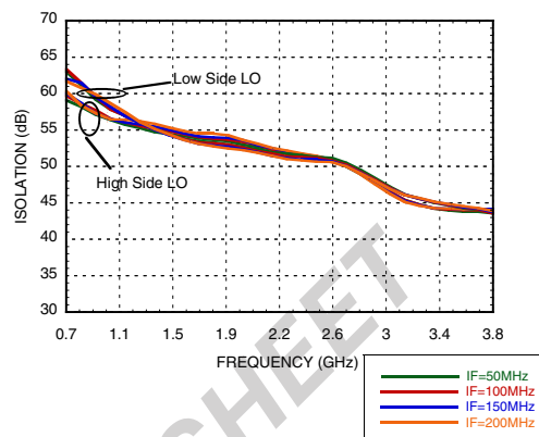
Figure 38. Channel to Channel Isolation vs. IF Frequency
