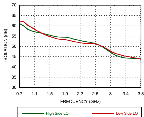
Figure 37. Channel to Channel Isolation vs. Frequency
