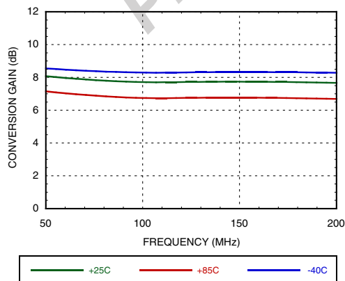
Figure 47. Conversion Gain vs. IF Frequency @ RF=2400 MHz, VGATE=5V [1]
