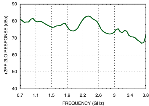
Figure 13. +2RF -2LO Response vs. Frequency over Temperature [1][2][3]
