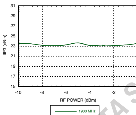
Figure 82. IIP3 vs. RF Input Power, RF= 1900 MHz, IF= 150 MHz, VGATE= 4.8V
