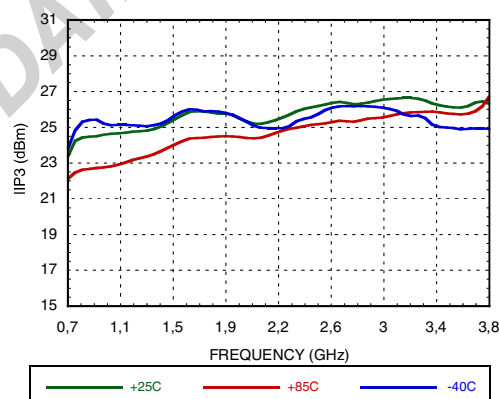
Figure 34. High Side LO Input IP3 vs. Frequency @ VGATE=4.8V [2]
