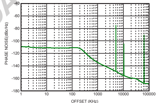
Figure 63. Fractional-N Spurious Performance @ 2646.96 MHz Exact Frequency Mode OFF [2]
