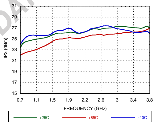
Figure 28. High Side LO Input IP3 vs. Frequency @ VGATE=4.9V [2]
