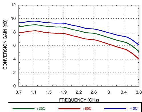
Figure 31. Low Side LO Conversion Gain vs. Frequency @ VGATE=4.8V [1][2]
