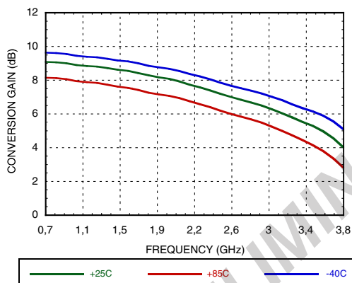
Figure 21. High Side LO Conversion Gain vs. Frequency @ VGATE=5V [1][2]
