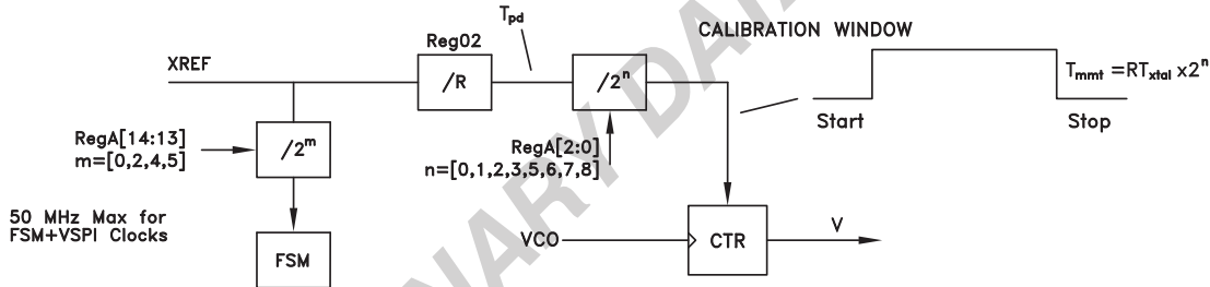
Figure 68. VCO Calibration
