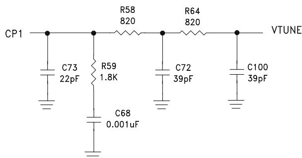
Figure 83. Loop filter components for HMC1190ALP6NE is configured as PLL alone used with external VCO HMC384LP4E
