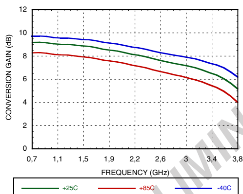
Figure 33. High Side LO Conversion Gain vs. Frequency @ VGATE=4.8V [1][2]
