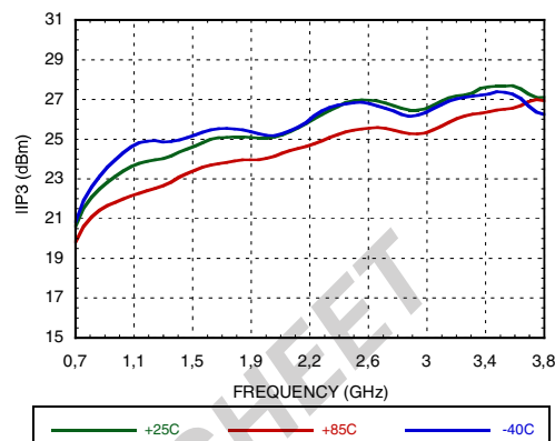
Figure 32. Low Side LO Input IP3 vs. Frequency @ VGATE=4.8V [2]
