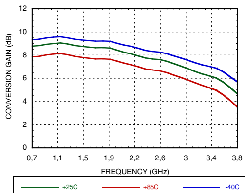
Figure 25. Low Side LO Conversion Gain vs. Frequency @ VGATE=4.9V [1][2]
