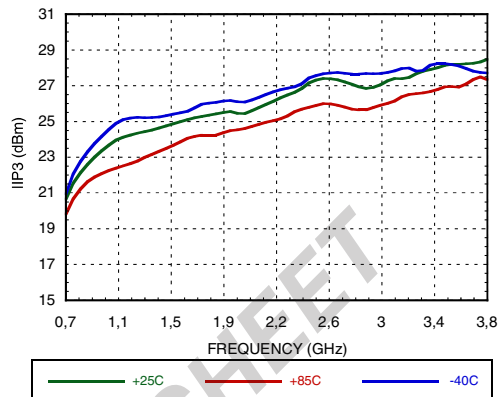
Figure 26. Low Side LO Input IP3 vs. Frequency @ VGATE=4.9V [2]
