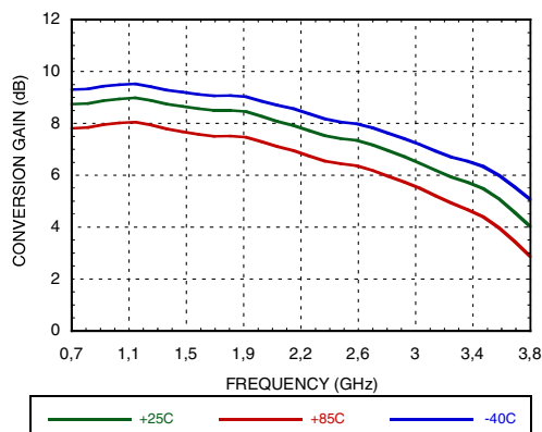
Figure 19. Low Side LO Conversion Gain vs. Frequency @ VGATE=5V [1][2]
