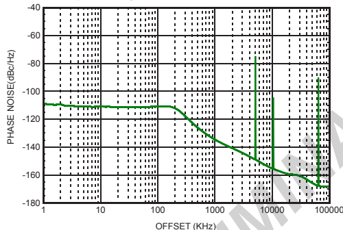
Figure 62. Fractional-N Spurious Performance @ 2646.96 MHz Exact Frequency Mode ON [2]
