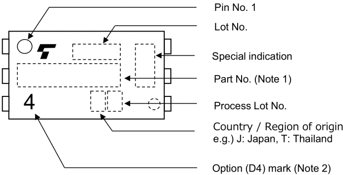
Fig. 17.4 Marking Example
