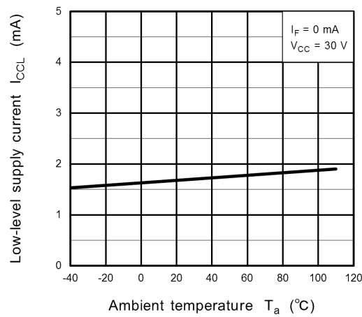
Fig. 13.2.5 I_{CCL} - T_a
