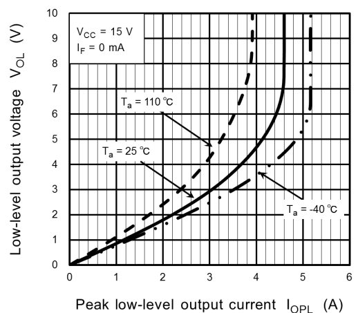
Fig. 13.2.9 V_{OL} - I_{OPL}
