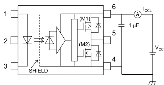
Fig. 13.1.6 I_{CCL} Test Circuit
