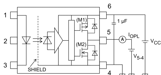
Fig. 13.1.2 I_{OPL} Test Circuit
