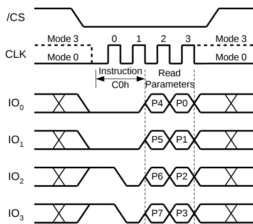
Figure 48b. Set Read Parameters Instruction (QPI Mode only)
