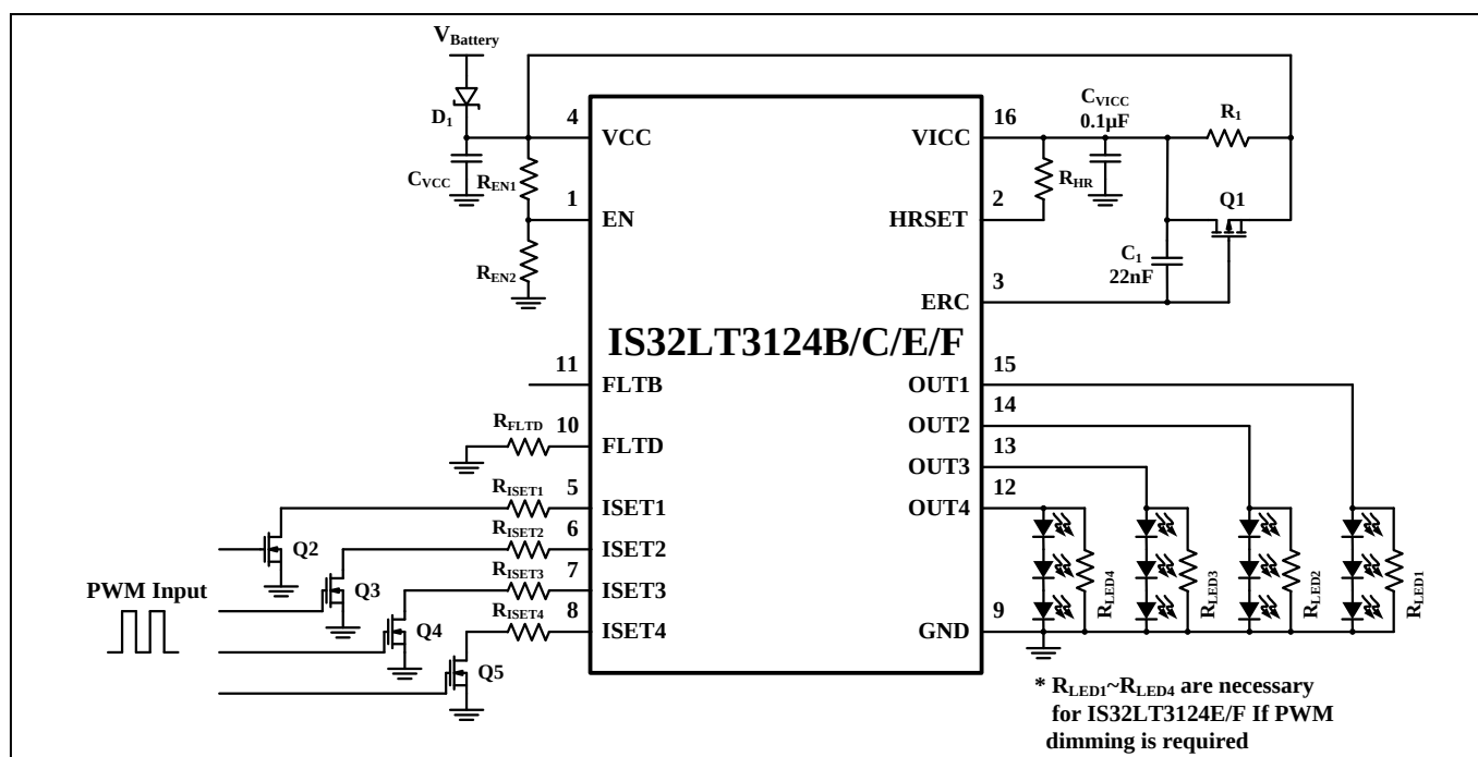
Figure 4 Typical Application Circuit with Additional Switches driving R SET Individual PWM Dimming (IS32LT3124B/C/E/F only) When PWM Generator is Far Away from Device
