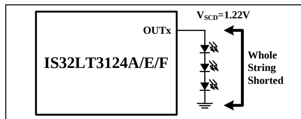
Figure 73 IS32LT3124A/E/F LED Short Detection
