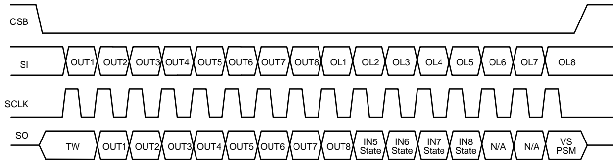
Figure 23. SPI Frame
