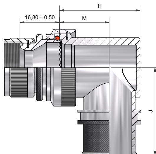
90° BACKSHELL - TYPE 2
