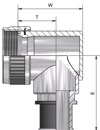
90° BACKSHELL - TYPE 1
