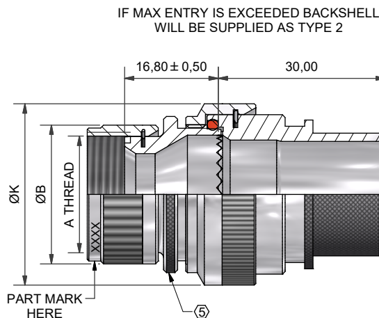
STRAIGHT BACKSHELL - TYPE 2
