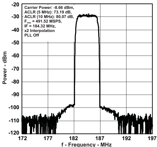
Figure 15. Single Carrier W-CDMA Test Model 1
