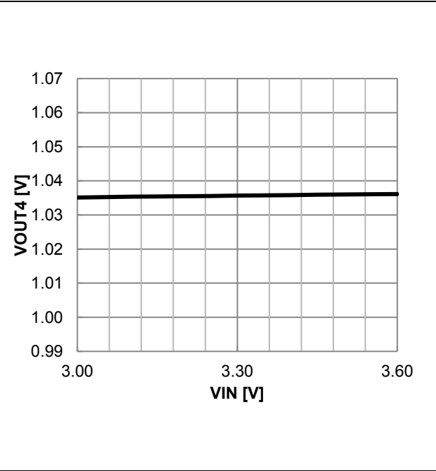
Figure 44. VOUT4 Output Voltage vs VIN
