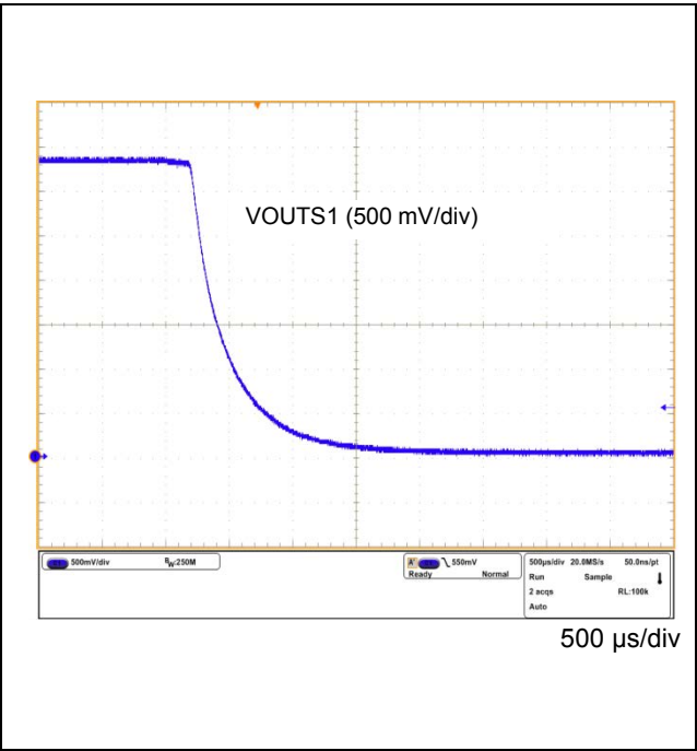
Figure 70. VOUTS1 Power OFF Waveform
