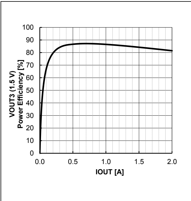
Figure 55. VOUT3 Power Efficiency vs IOUT (VOUT3 = 1.5 V Setting)
