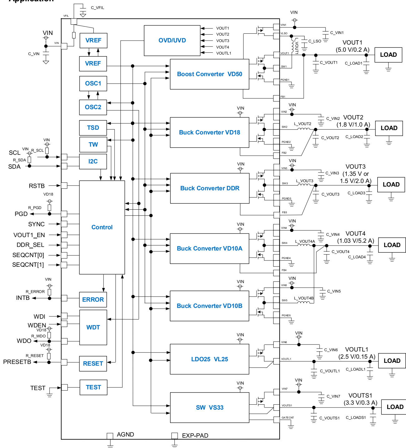
Figure 2. Application Circuit
