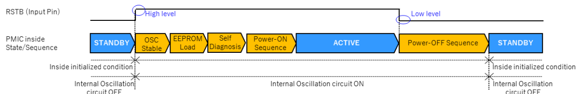
Figure 4. RSTB Operation Timing Chart
