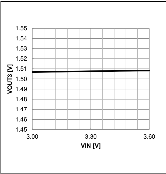
Figure 43. VOUT3 Output Voltage vs VIN (VOUT3 = 1.5 V Setting)
