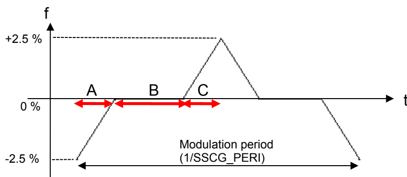
Figure 39. Modulation Waveform of SSCG
