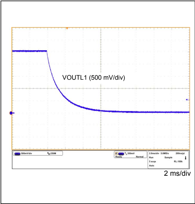
Figure 69. VOUTL1 Power OFF Waveform
