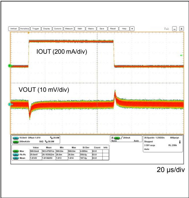
Figure 72. VOUT2 Load Transient (IOUT = 0 A to 0.5 A (SR = 1 A/ \mu s))
