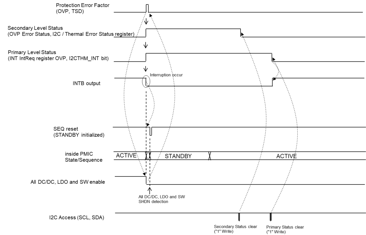
Figure 33. Timing Chart when Protection Error Factor Occur 2
