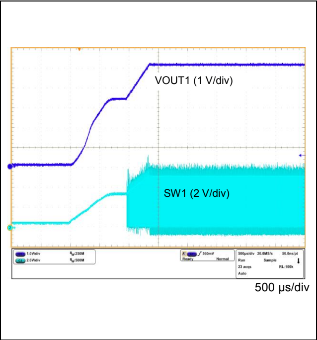
Figure 57. VOUT1 Power ON Waveform
