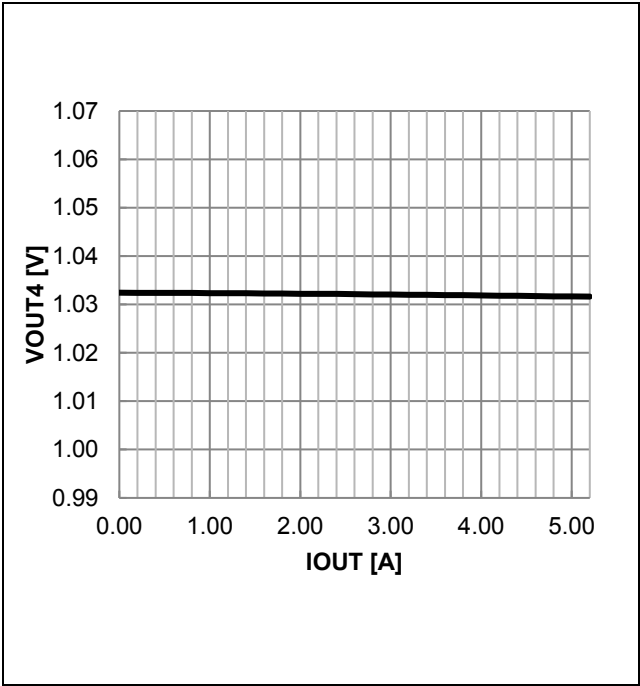
Figure 50. VOUT4 Output Voltage vs IOU
