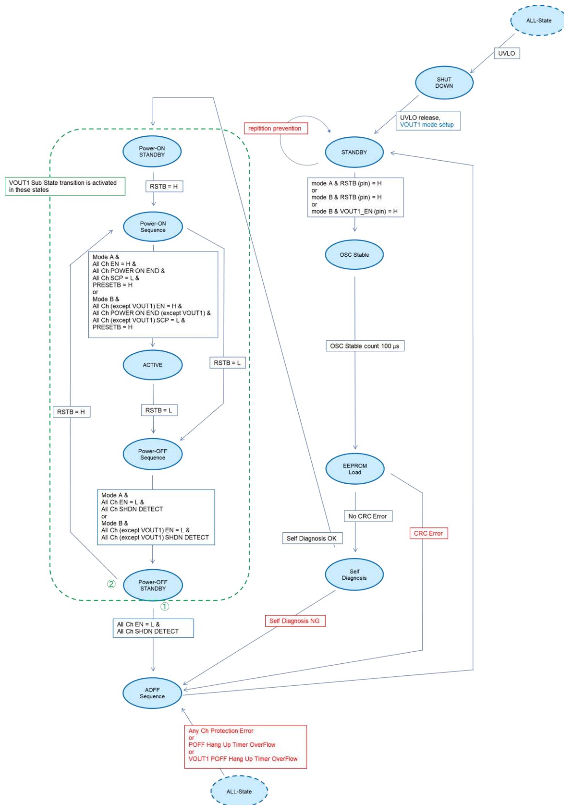
Figure 12. Main State Machine
