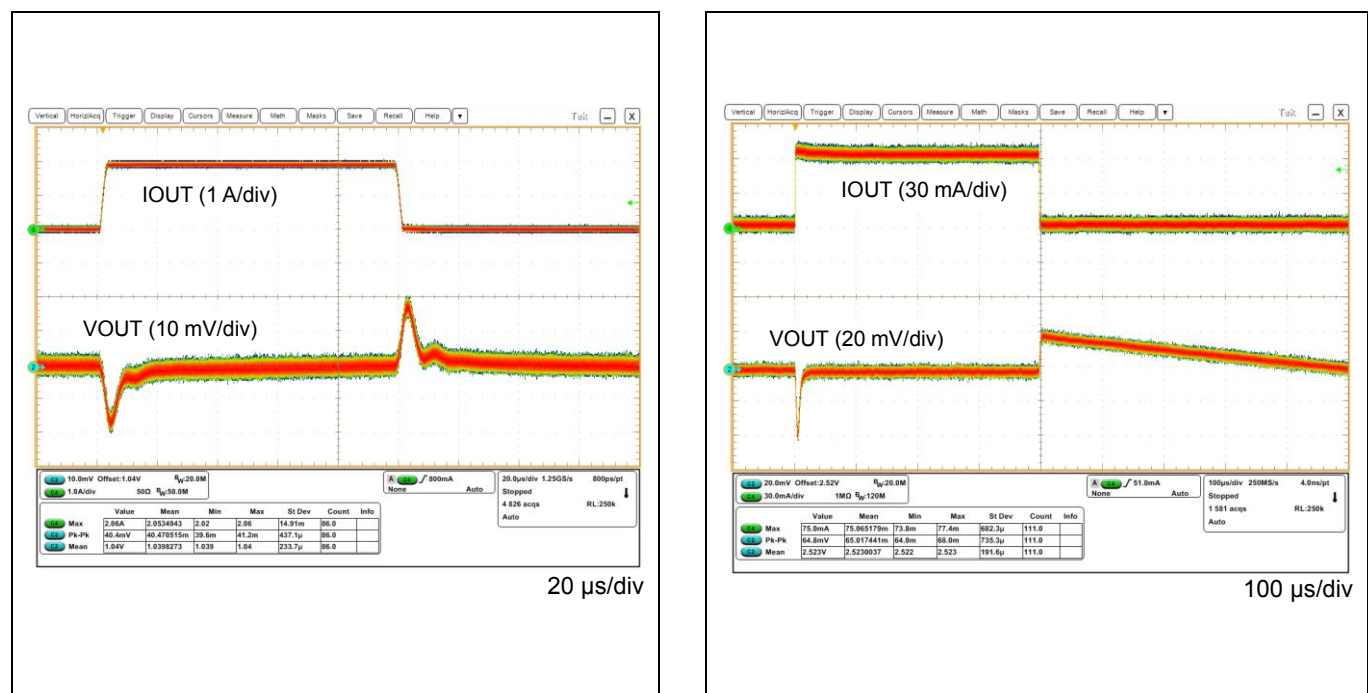
Figure 75. VOUT4 Load Transient (IOUT = 0 A to 2.05 A (SR = 1 A/ \mu s)) Figure 76. VOUTL1 Load Transient (IOUT = 0 A to 75 mA (SR = 100 mA/ \mu s))
