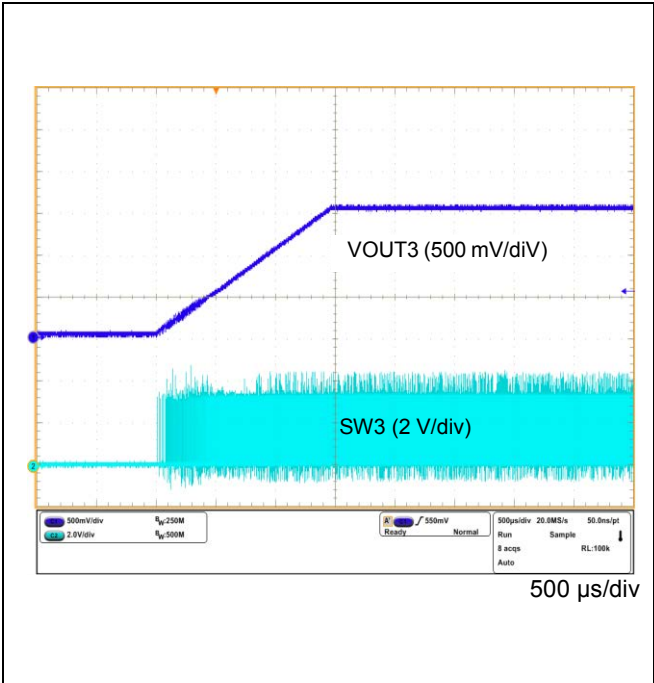
Figure 60. VOUT3 Power ON Waveform (VOUT3 = 1.5 V Setting)
