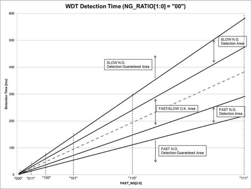
Figure 37. WDT Detection Time when NG_RATIO[1:0] = "00"
