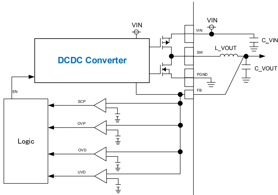
Figure 31. Power Abnormality Monitoring Circuit
