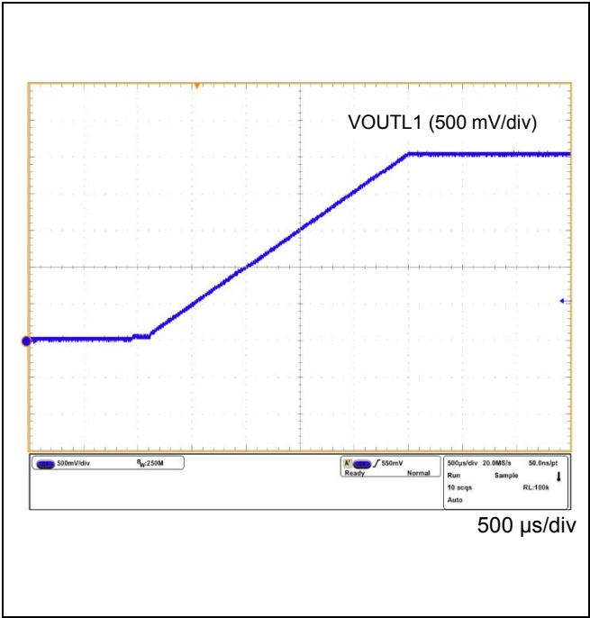
Figure 62. VOUTL1 Power ON Waveform
