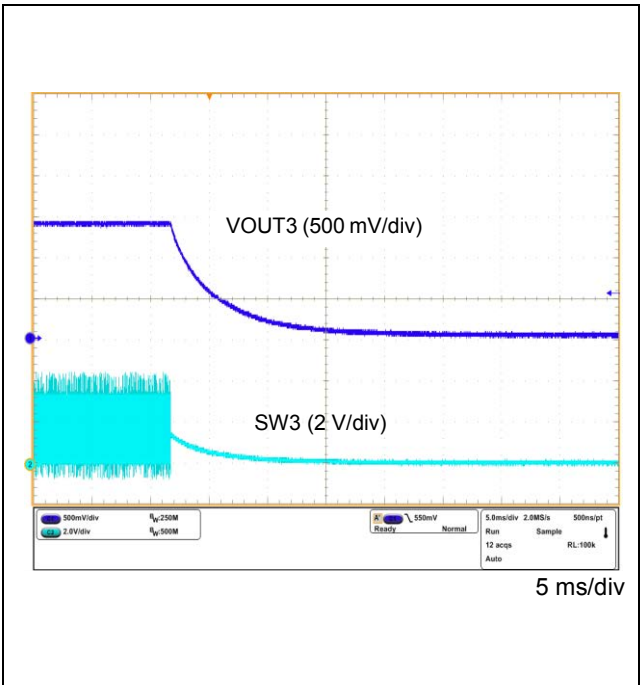
Figure 66. VOUT3 Power OFF Waveform (VOUT3 = 1.35 V Setting)
