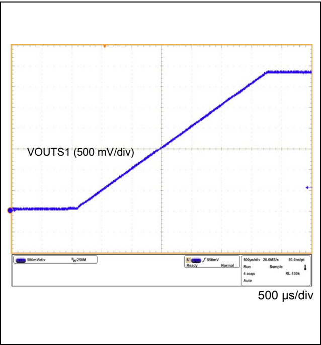
Figure 63. VOUTS1 Power ON Waveform
