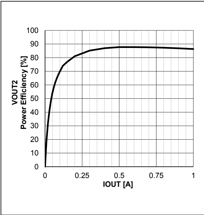
Figure 53. VOUT2 Power Efficiency vs IOUT
