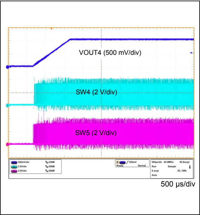
Figure 61. VOUT4 Power ON Waveform
