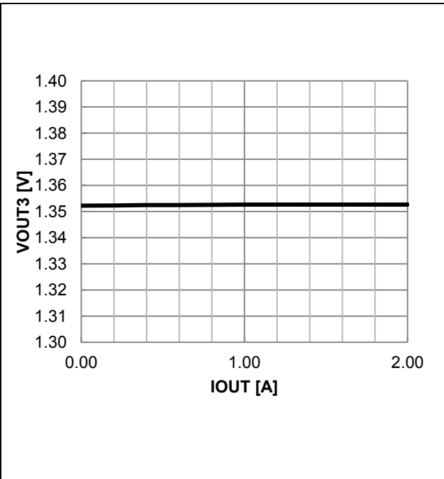
Figure 48. VOUT3 Output Voltage vs IOU (VOUT3 = 1.35 V Setting)
