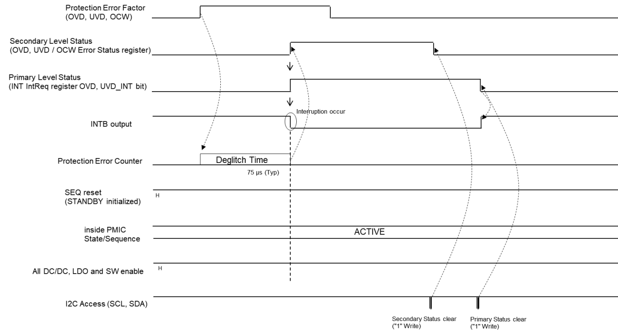
Figure 34. Timing Chart when Protection Detection Factor Occur
