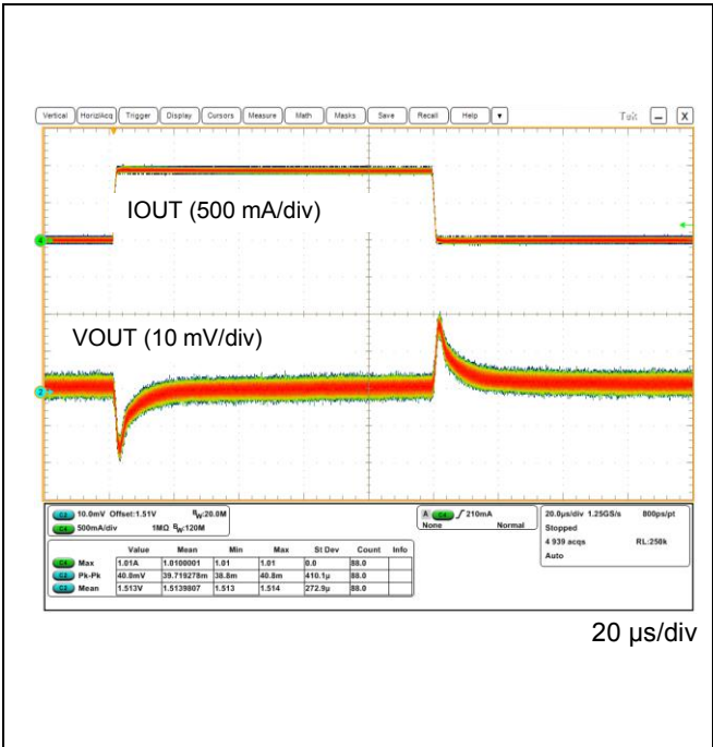
Figure 74. VOUT3 Load Transient (VOUT3 = 1.5 V Setting, IOUT = 0 A to 1 A (SR = 1 A/ \mu s))
