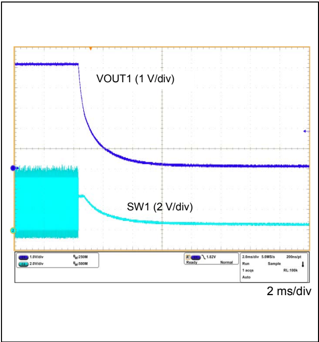
Figure 64. VOUT1 Power OFF Waveform
