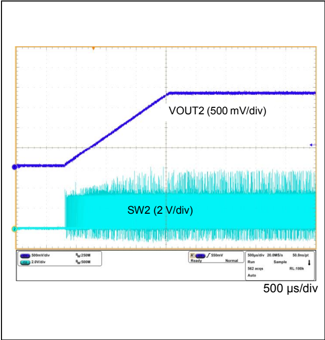
Figure 58. VOUT2 Power ON Waveform
