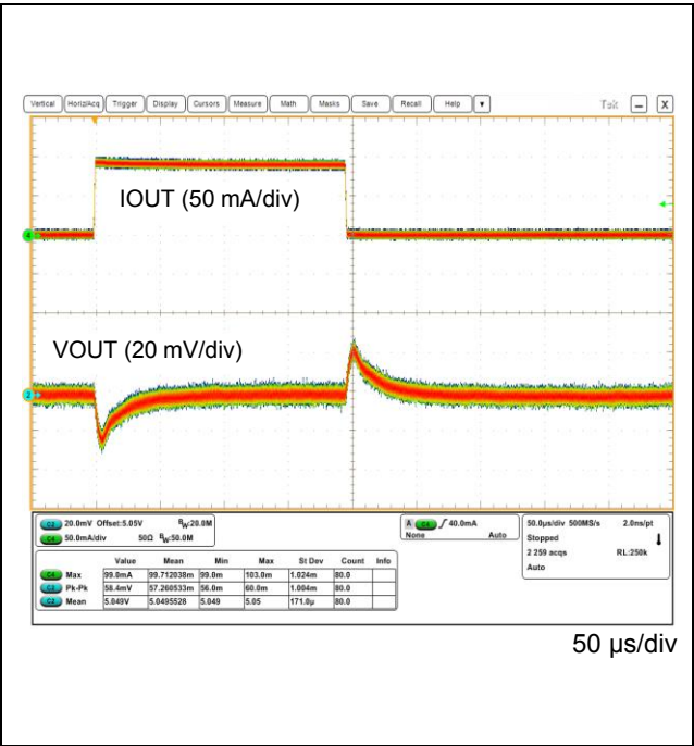
Figure 71. VOUT1 Load Transient (IOUT = 0 A to 100 mA (SR = 100 mA/ \mu s))
