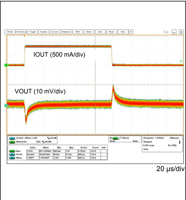
Figure 73. VOUT3 Load Transient (VOUT3 = 1.35 V Setting, IOUT = 0 A to 1 A (SR = 1 A/ \mu s))
