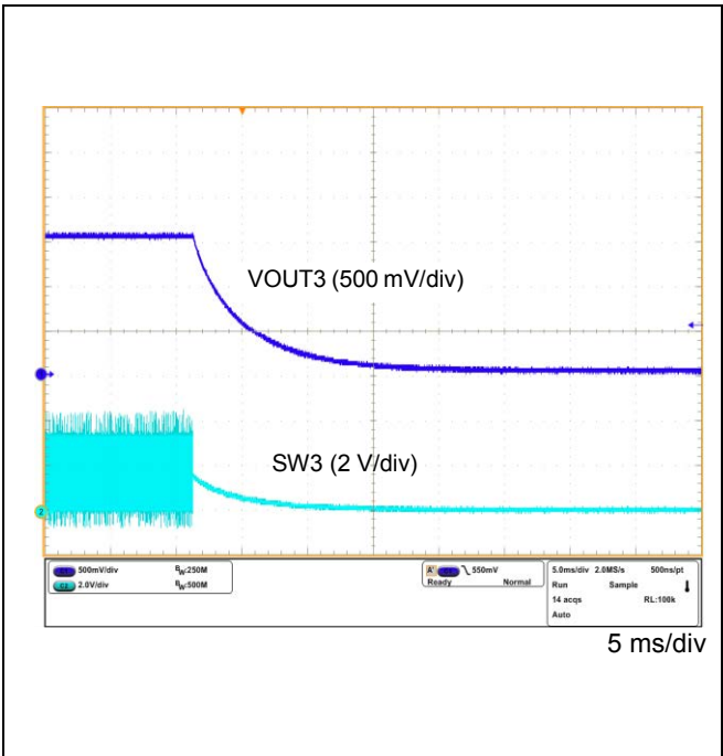
Figure 67. VOUT3 Power OFF Waveform (VOUT3 = 1.5 V Setting)
