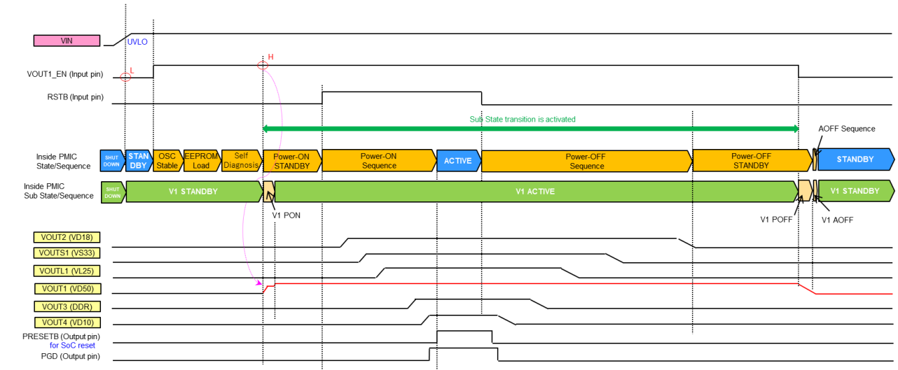
Figure 9. Whole Sequence1 (Mode B)
