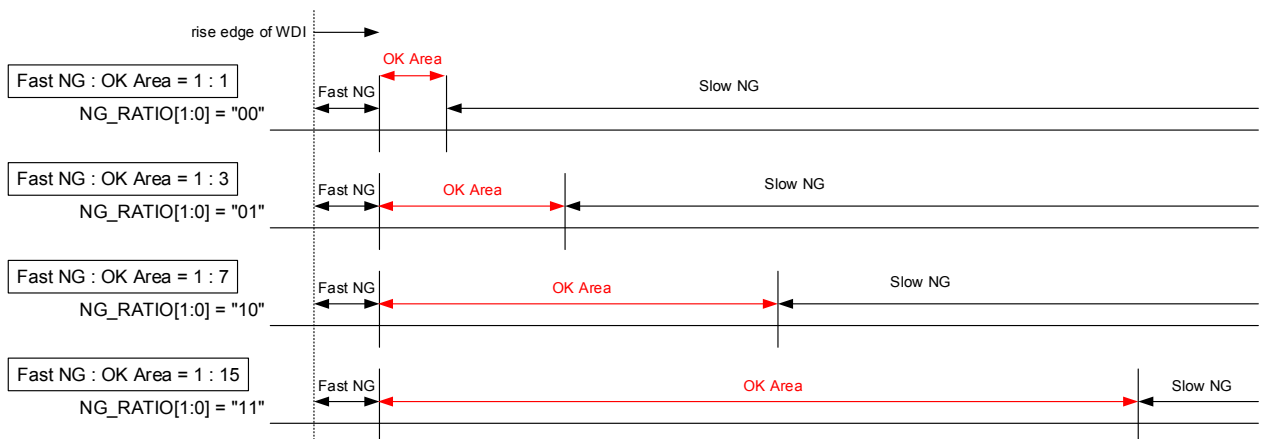
Figure 36. WDT NG RATIO
