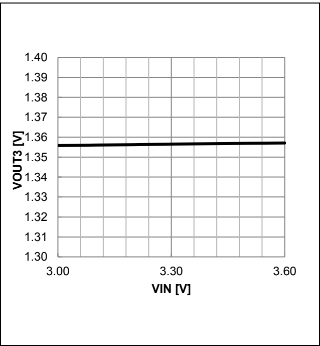
Figure 42. VOUT3 Output Voltage vs VIN (VOUT3 = 1.35 V Setting)
