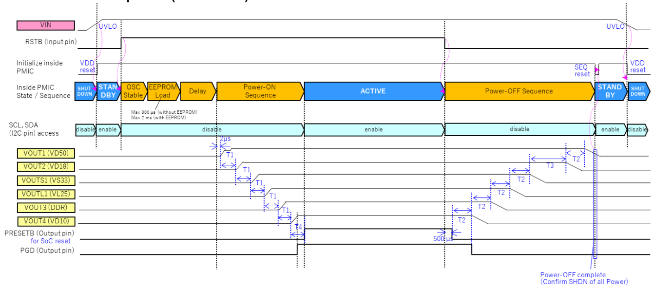
Figure 14. Whole Sequence (State Chart)
