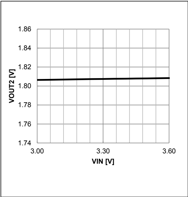
Figure 41. VOUT2 Output Voltage vs VIN
