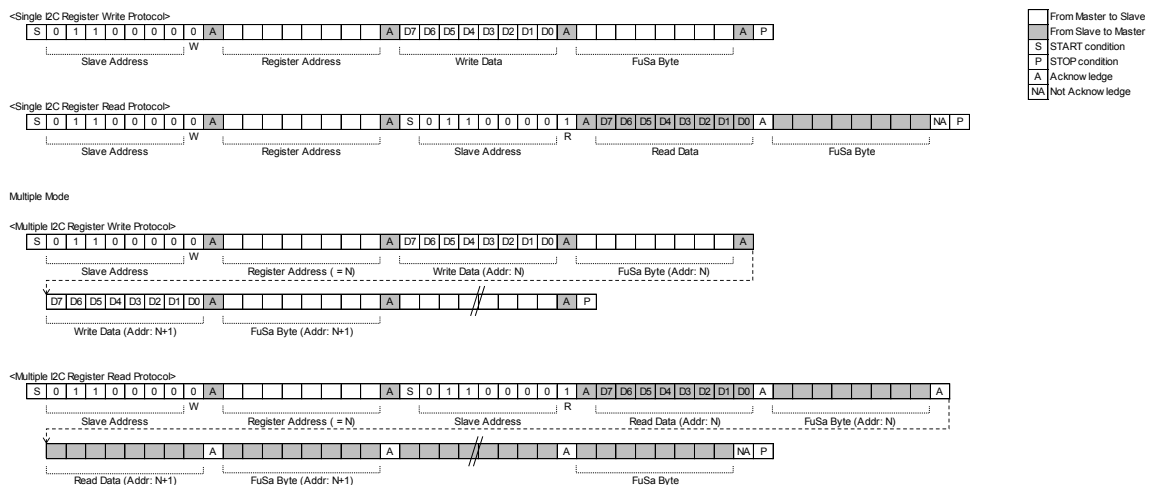
Figure 24. I2C Protocol (FuSa Mode)
