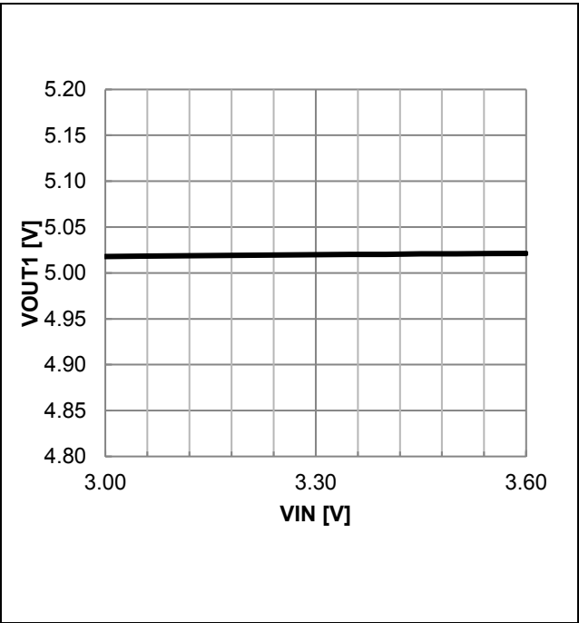
Figure 40. VOUT1 Output Voltage vs VIN
