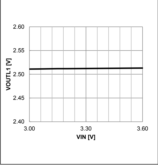
Figure 45. VOUTL1 Output Voltage vs VIN
