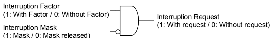
Figure 28. Interruption Factor/Mask/Request
