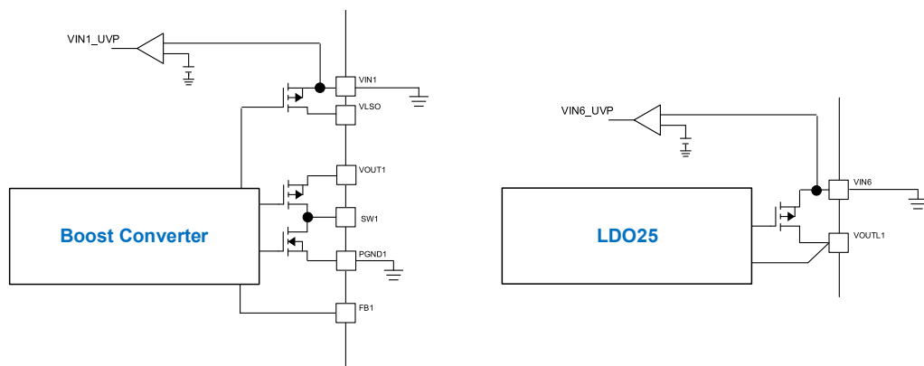
Figure 18. VOUT1, VOUTL1 OFF Circuit
