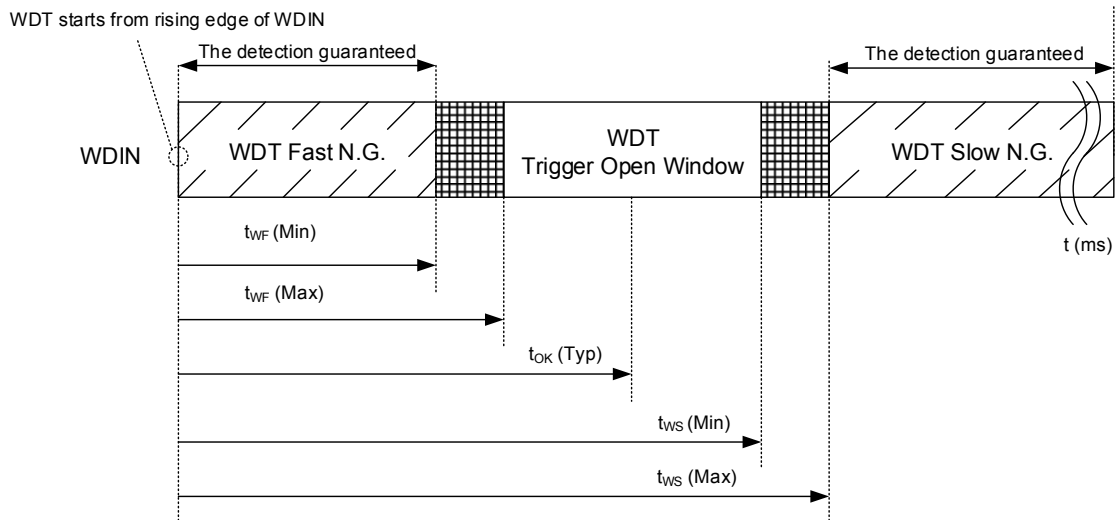
Figure 35. WDT Function
