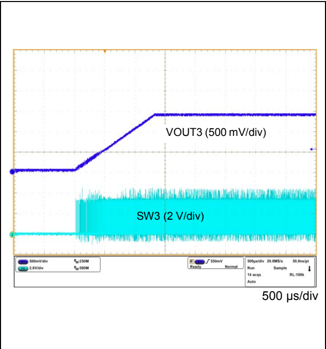
Figure 59. VOUT3 Power ON Waveform (VOUT3 = 1.35 V Setting)
