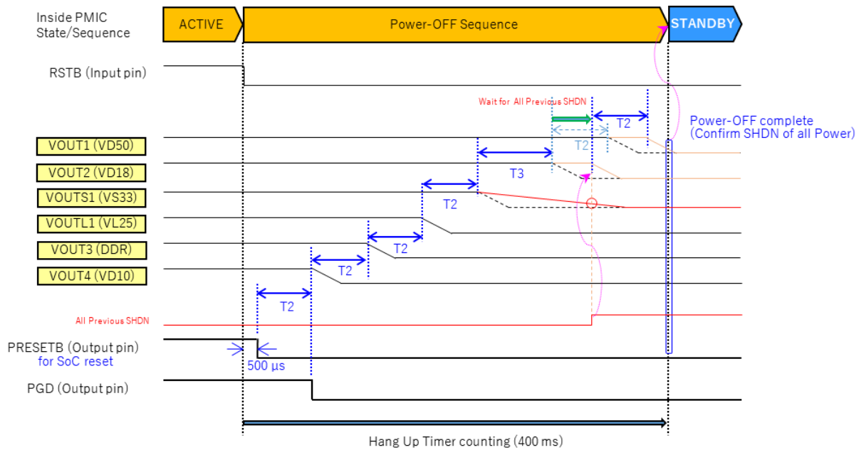
Figure 7. VOUT2 Discharge Start Timing
