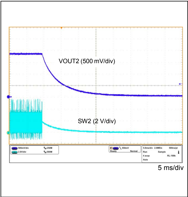
Figure 65. VOUT2 Power OFF Waveform
