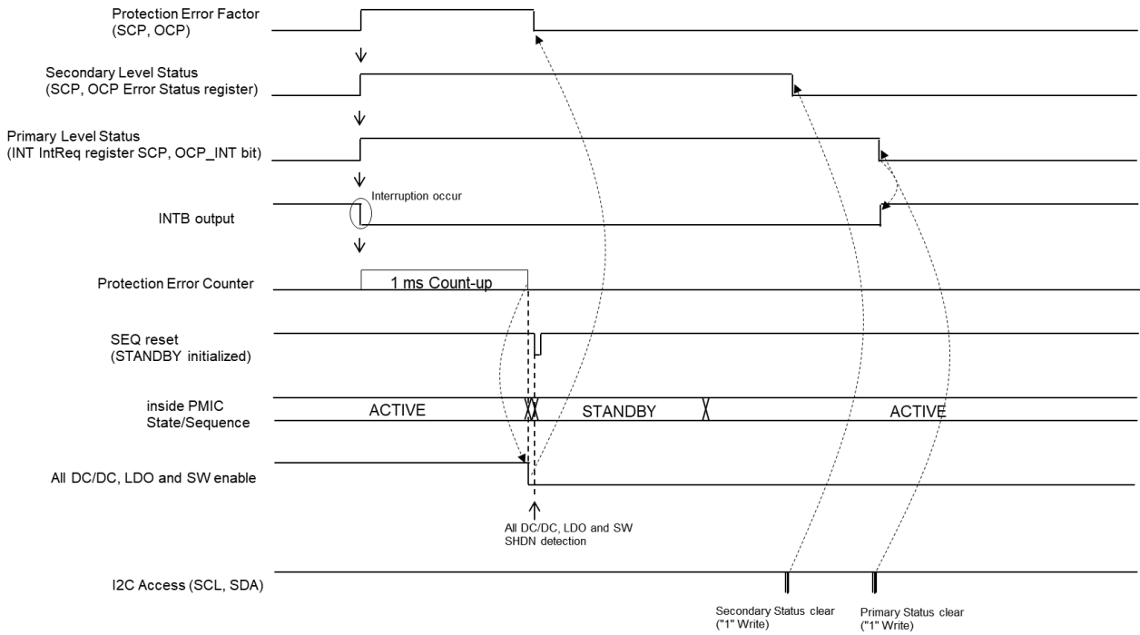
Figure 32. Timing Chart when Protection Error Factor Occur 1
