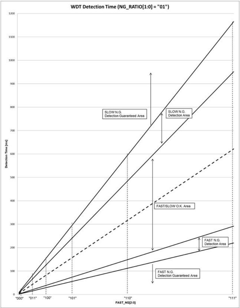
Figure 38. WDT Detection Time when NG_RATIO[1:0] = "01"
