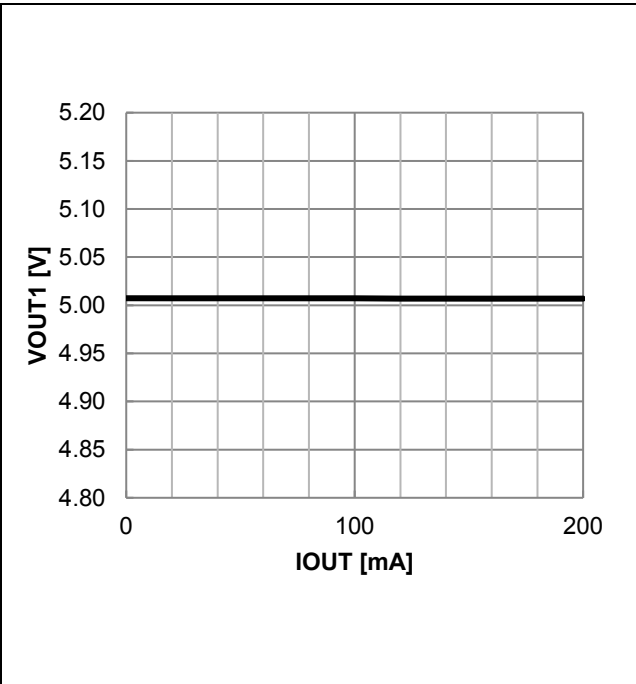
Figure 46. VOUT1 Output Voltage vs IOU
