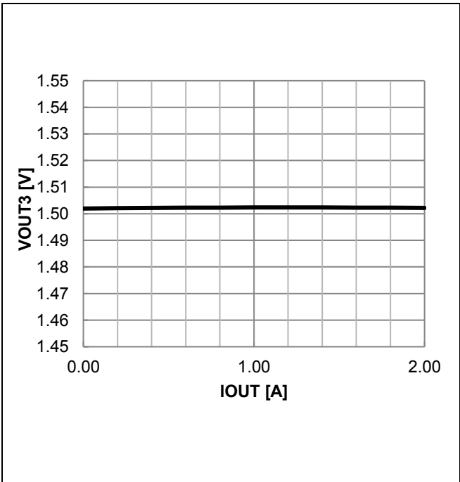
Figure 49. VOUT3 Output Voltage vs IOU (VOUT3 = 1.5 V Setting)
