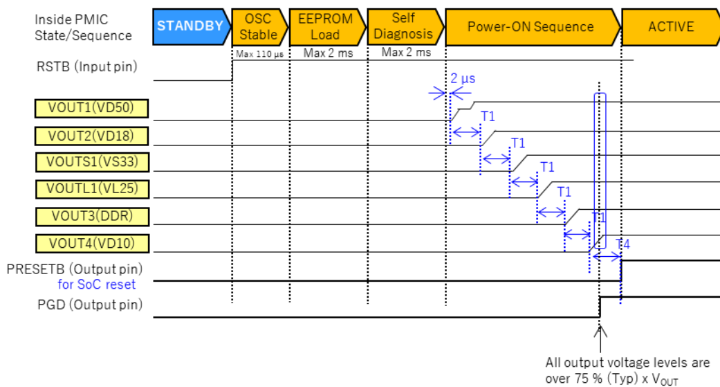
Figure 5. Output Power-ON Operation Timing Chart (Default Register Setting)
