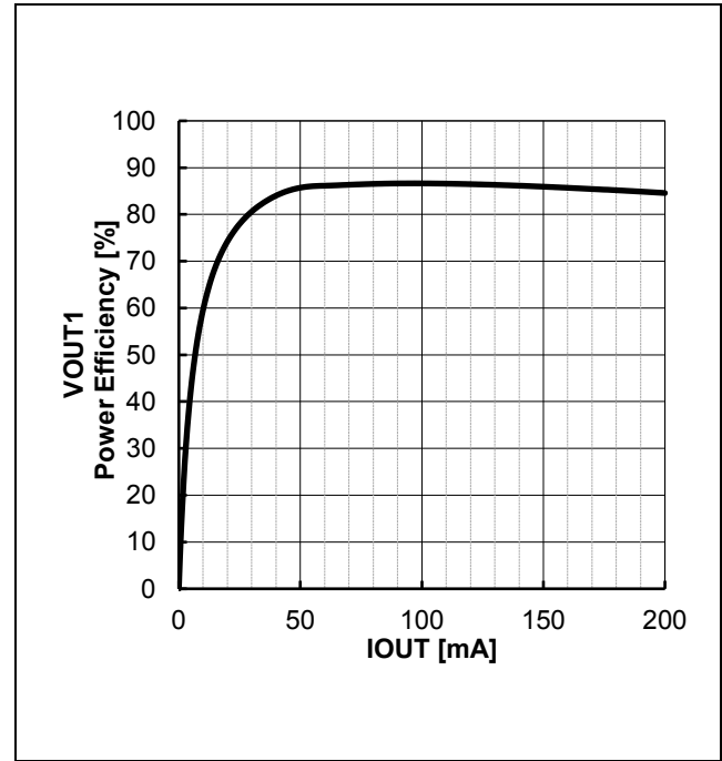
Figure 52. VOUT1 Power Efficiency vs IOUT
