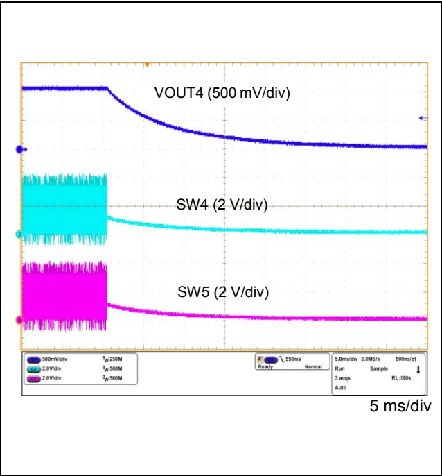
Figure 68. VOUT4 Power OFF Waveform
