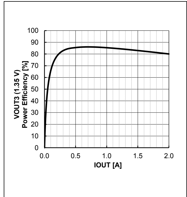
Figure 54. VOUT3 Power Efficiency vs IOUT (VOUT3 = 1.35 V Setting)
