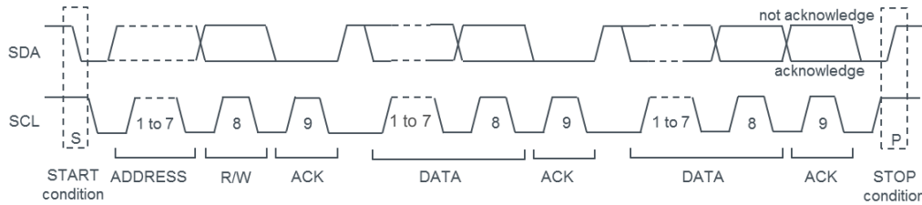
Figure 22. I2C Basic Protocol
