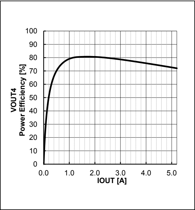
Figure 56. VOUT4 Power Efficiency vs IOU
