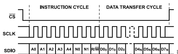
Figure 88. Serial Register Interface Timing, LSB First Read
