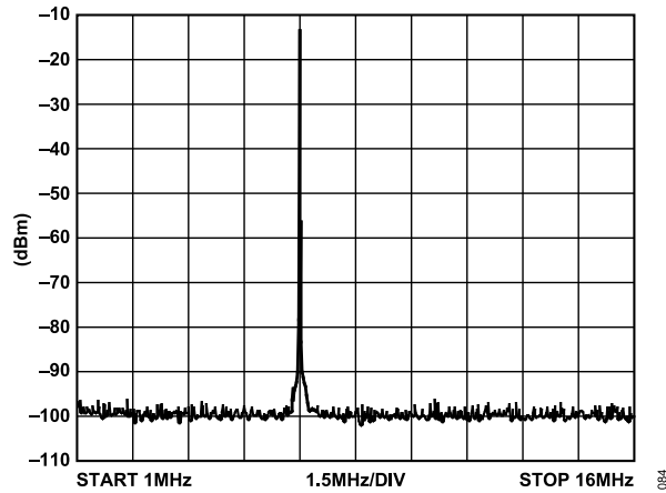
Figure 54. AD9717 Single-Tone Spectrum, 1.8 V
