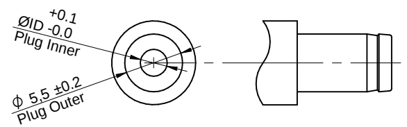
Recommended DC mate plug
