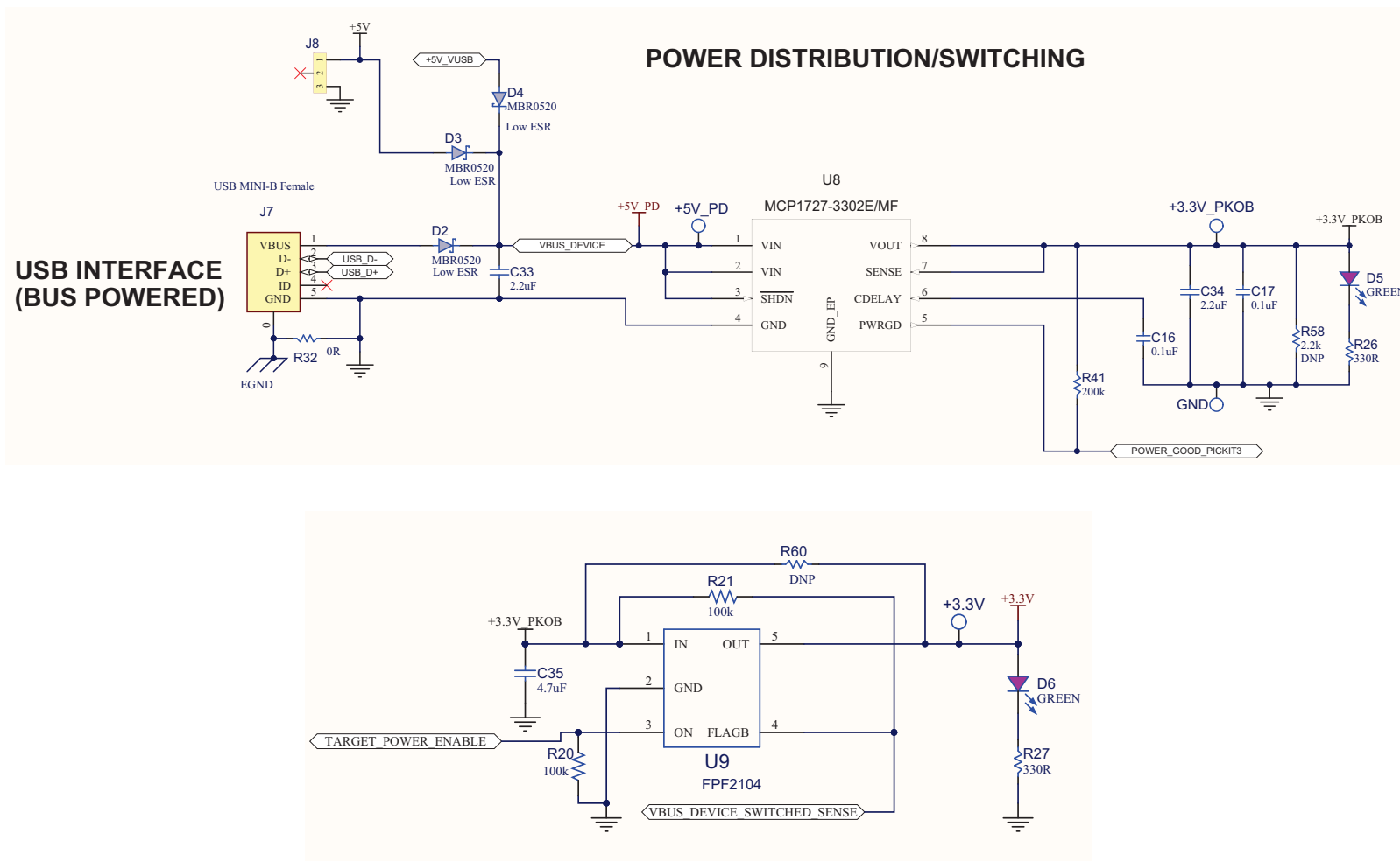
FIGURE A-9: POWER DISTRIBUTION (SHEET 1 OF 2)
