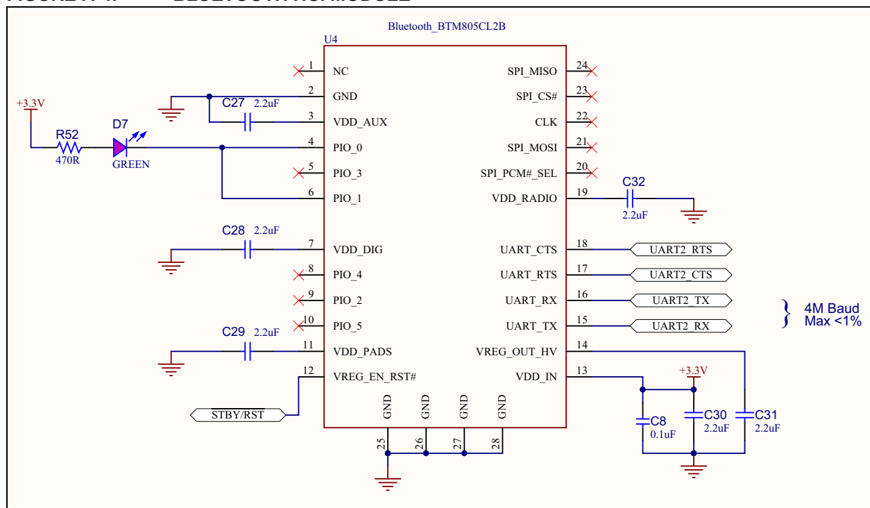
FIGURE A-4: BLUETOOTH HCI MODULE
