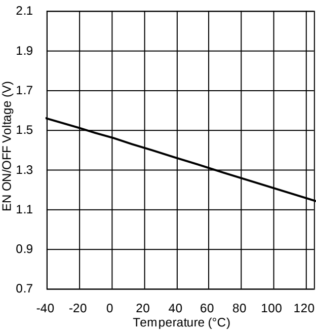
Figure 5. EN ON/OFF Voltage vs Temperature
