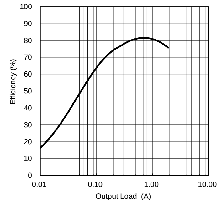
Figure 19. Efficiency vs Output Load
