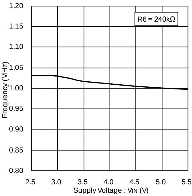
Figure 7. Frequency vs Supply Voltage
