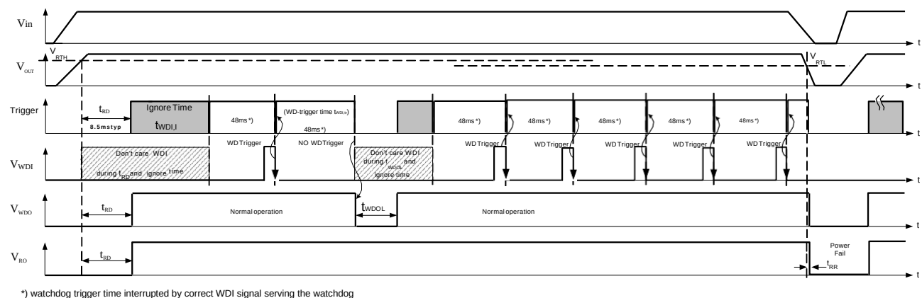
Typical Watchdog Timing Diagram, Watchdog and Reset Modes
