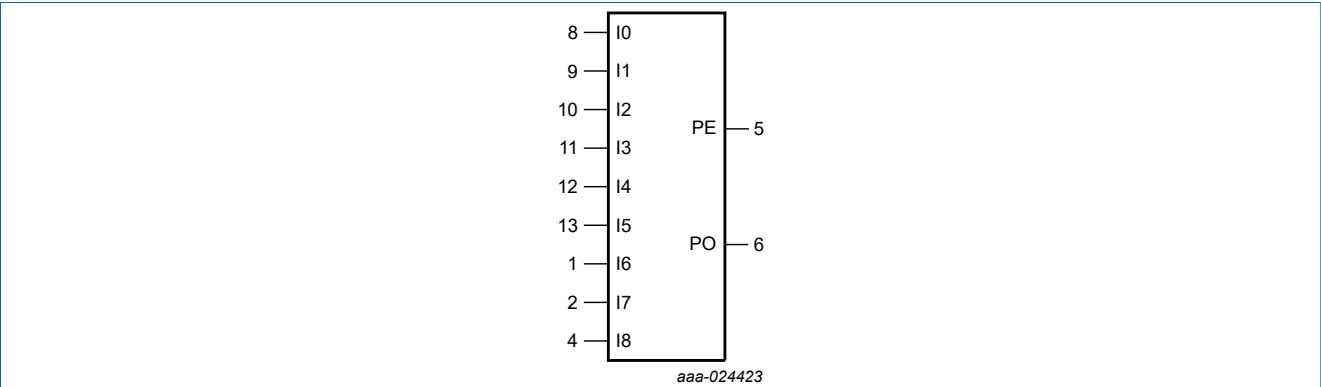
Fig. 1. Logic symbol
