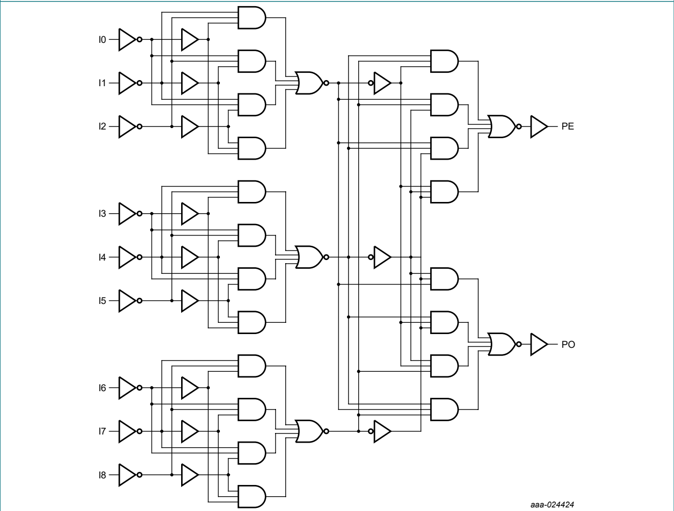
Fig. 2. Logic diagram
