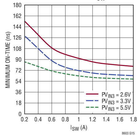
Channel 3 Minimum On-Time vs I_{SW}
