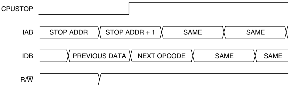
Figure 6-18. Stop Mode Entry Timing
