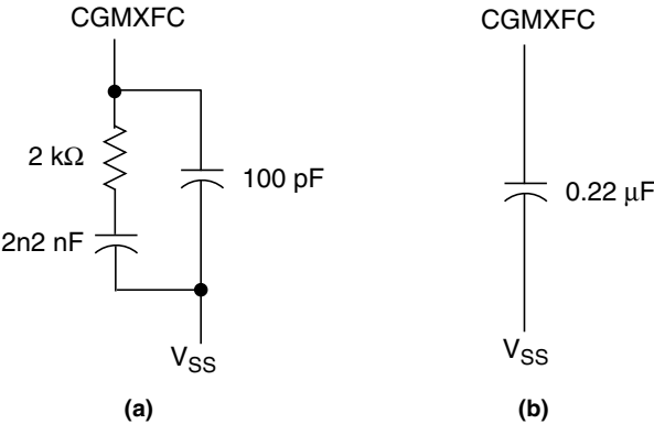
Figure 5-10. PLL Filter
