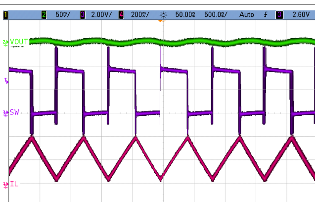
Figure 9-16. PWM Mode Operation
