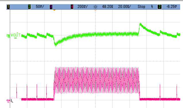
Figure 9-20. Load Transient Response; 5 mA to 290 mA
