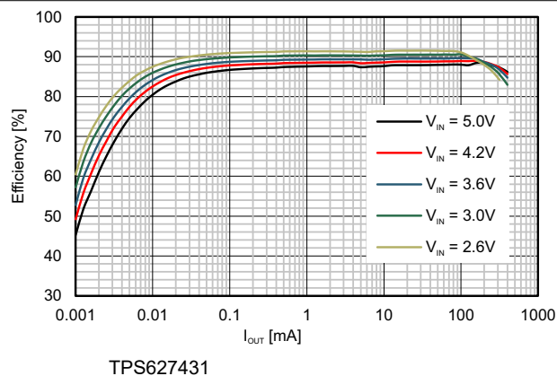
Figure 9-5. Efficiency vs Load Current; V_{OUT} = 1.9\text{ V}
