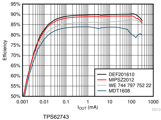
Figure 9-9. Efficiency vs Load Current; V_{OUT} = 1.8\text{ V}
