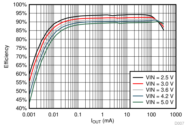
Figure 9-4. Efficiency vs Load Current; V_{OUT} = 2.1\text{ V}
