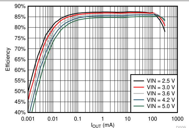
Figure 9-6. Efficiency vs Load Current; V_{OUT} = 1.8\text{ V}
