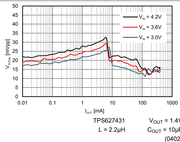
Figure 9-14. Typical Output Ripple Voltage V_{OUT} = 1.4\text{ V}
