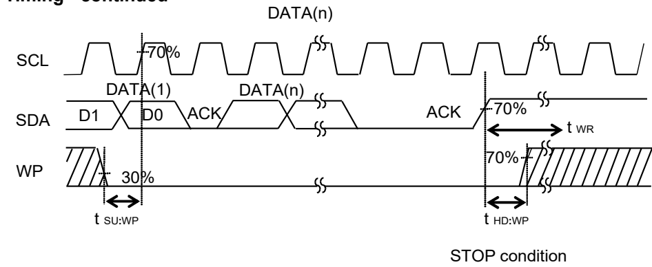
Figure 5-(d). WP Timing at Write Execution
