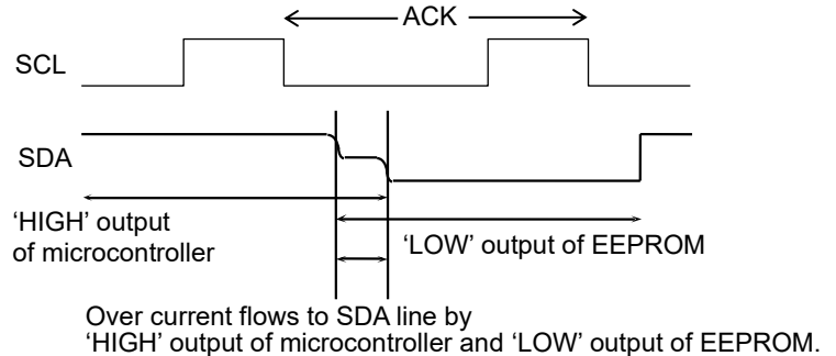
Figure 53. I/O Collision Timing
