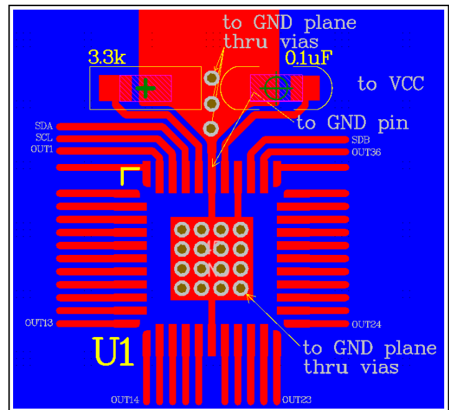
Figure 7 Layout Example
