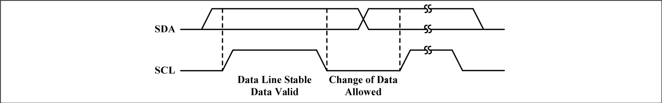
Figure 3 Bit Transfer
