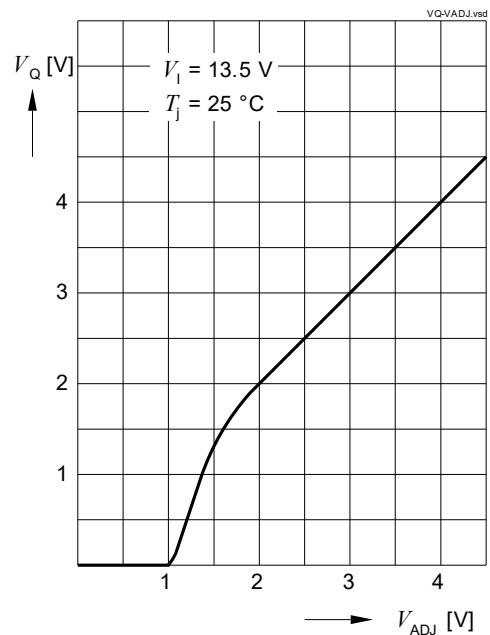
Output voltage V_Q vs. adjust voltage V_{ADJ,EN}
