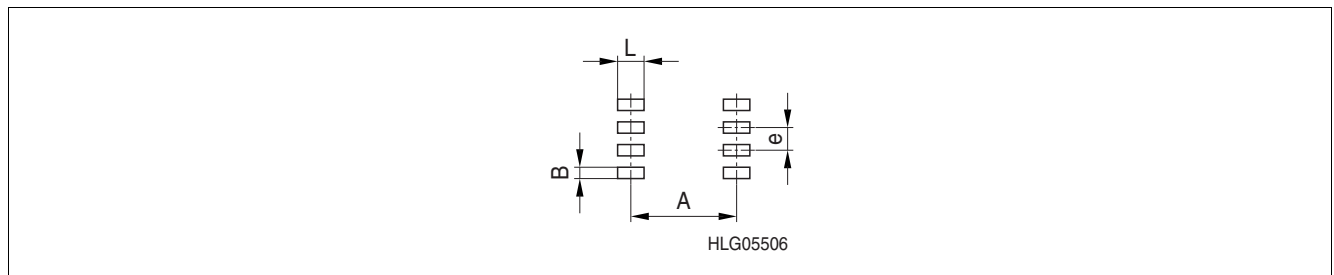
Figure 9 Footprint PG-DSO-8
