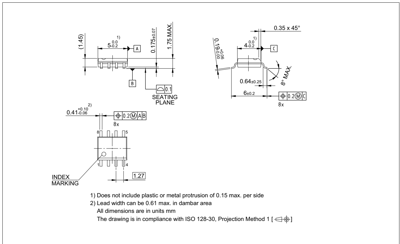
Figure 8 Outline PG-DSO-8
