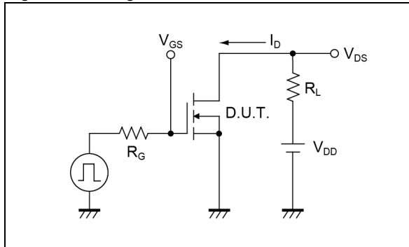
Fig.1-1 Switching Time Measurement Circuit
