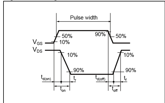
Fig.1-2 Switching Waveforms
