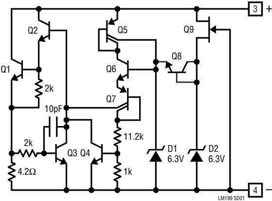
Temperature Stabilizer
