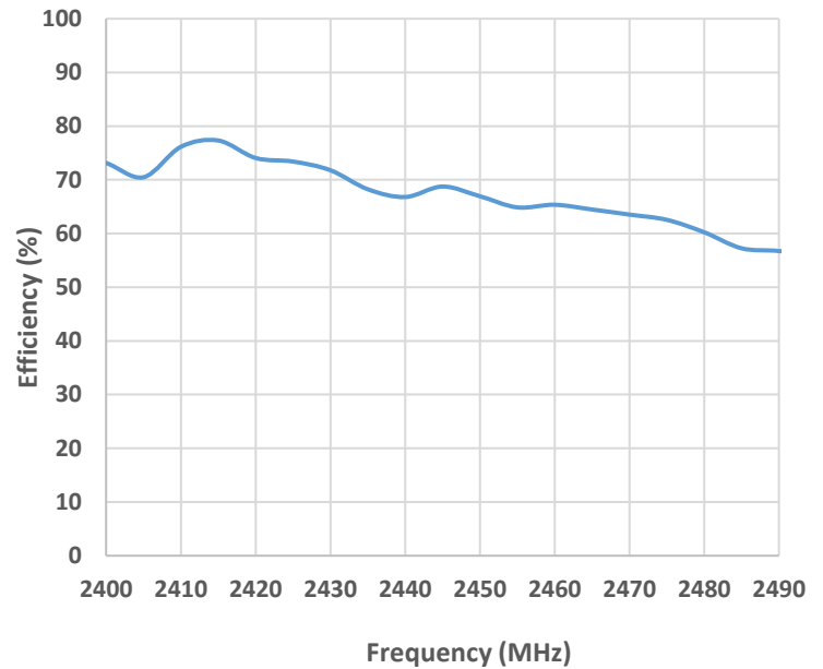
Efficiency (2400 – 2490 MHz)
