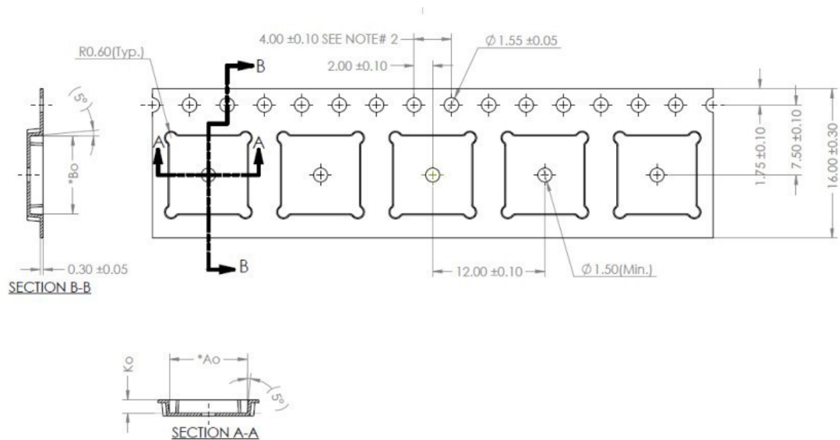
Figure 6-2. Tape Specifications
