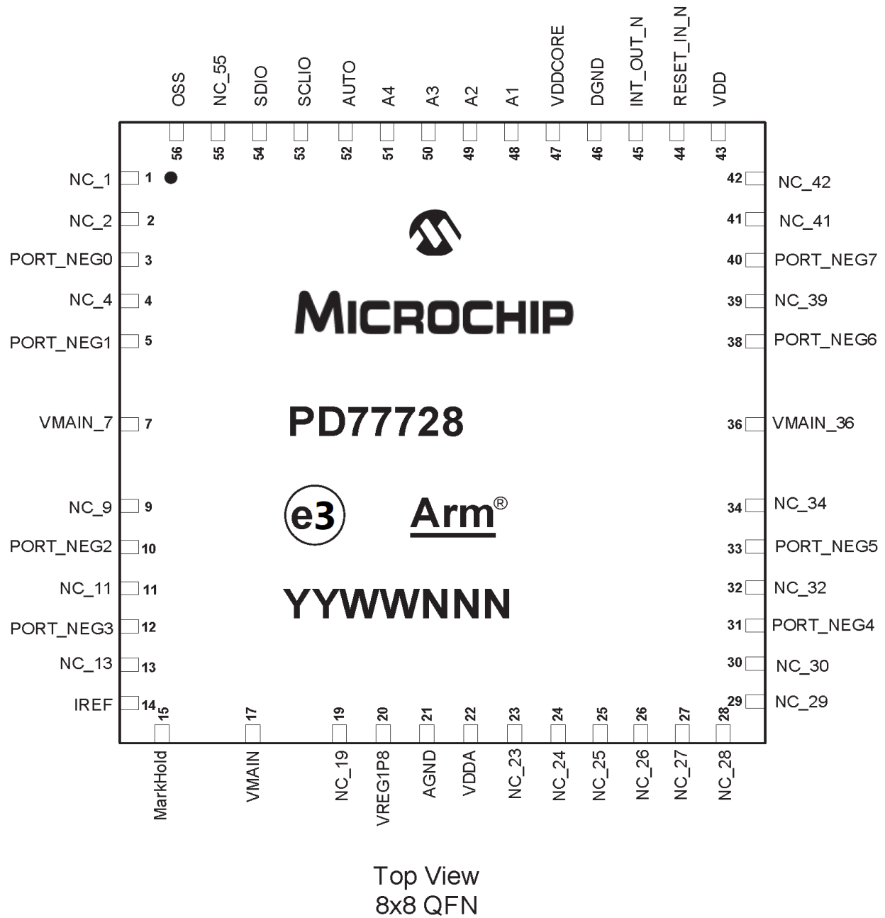
Figure 3-1. Pinout
