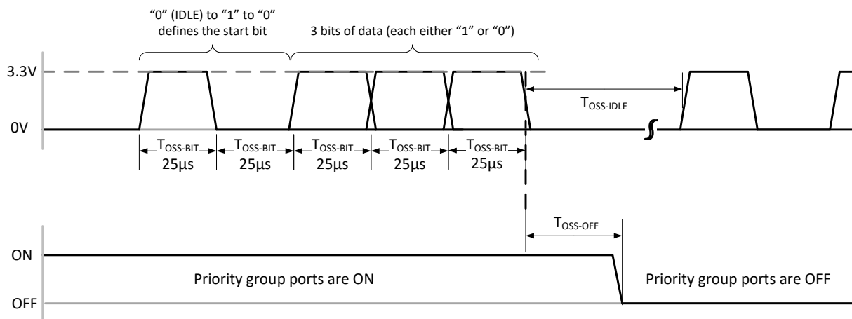
Figure 4-5. OSS Pin Multi-Bit Priority Shutdown Mode Timing
