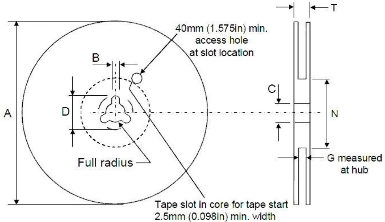
Figure 6-3. Reel Specification
