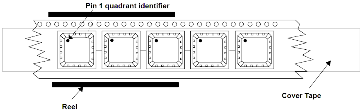
Figure 6-2. Tape Specifications
