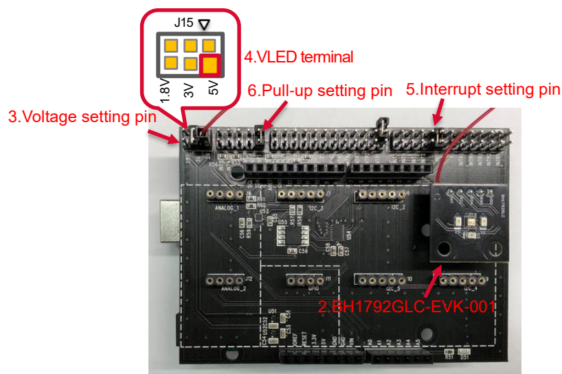
Figure 2. Connection between BH1792GLC-EVK-001 and the SensorShield
