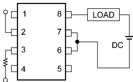
Fig. 14.2.2 B Connection
