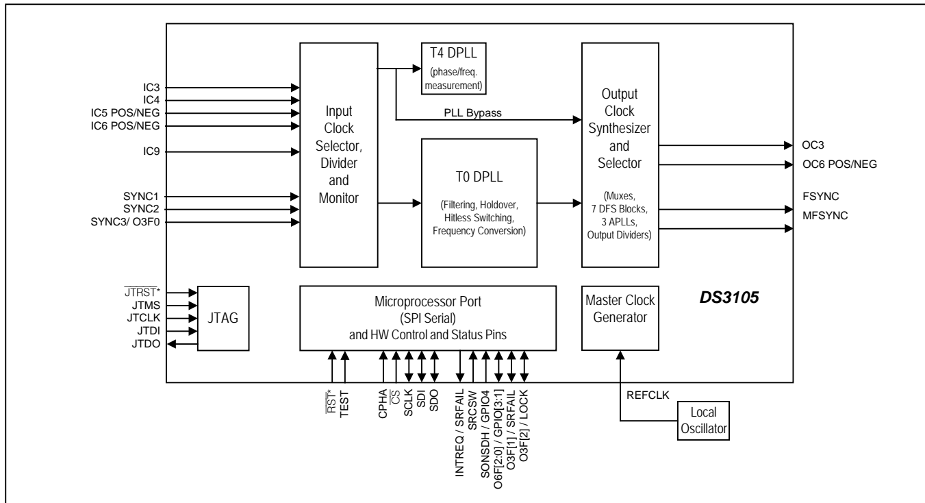
Figure 3-1. Block Diagram
