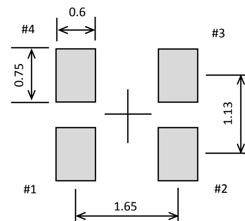
[ 8 ] Recommended foot print unit:mm
