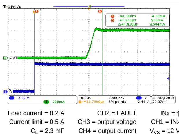
Figure 39. Driving a Capacitive Load, Expanded Waveform
