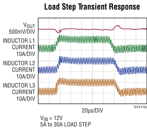
Figure 10. High Efficiency 380kHz 3-Phase 5V/50A Regulator
