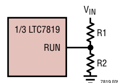
Figure 5. Using the RUN Pins As a UVLO
