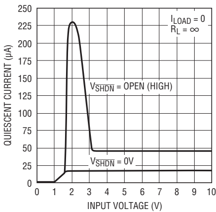
LT1529-3.3 Quiescent Current
