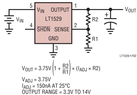
Figure 2. Adjustable Operation
