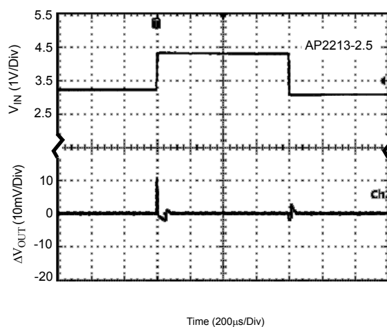
Figure 11. Line Transient (Conditions: V_{IN} = 3.4 to 4.4V , V_{EN} = 2V , I_{OUT} = 100\mu A , C_{BYP} = 100pF , C_{OUT} = 2.2\mu F )
