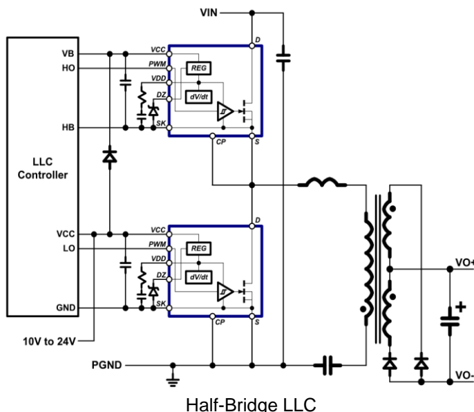
Half-Bridge LLC
