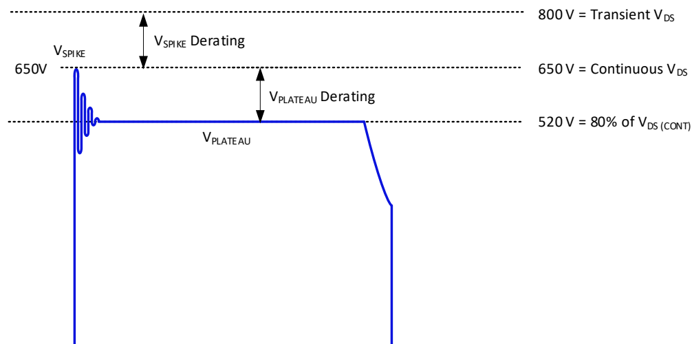
Fig. 27 QR flyback drain-to-source voltage stress diagram
