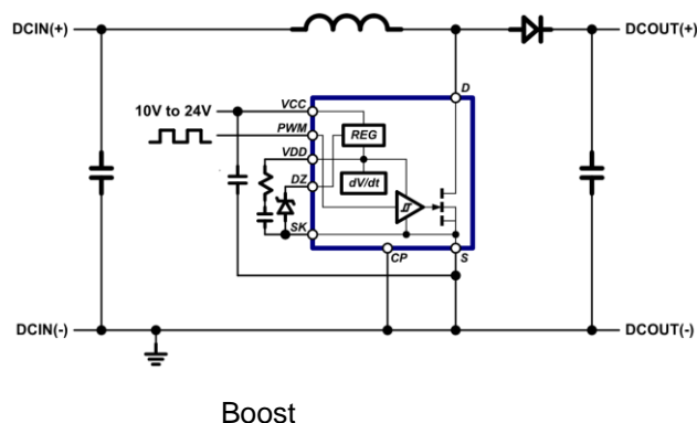
Boost
