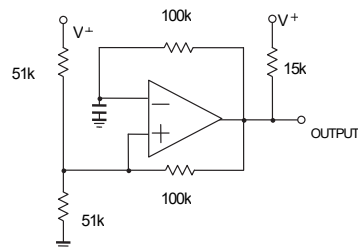
Pulse Generator
