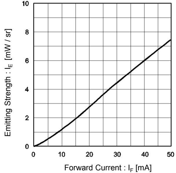
Fig.3 Emitter Strength vs. Forward Current
