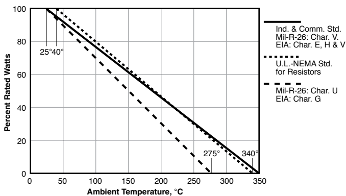
Fig. 4: Derating of Resistors for High Ambient Temperatures.
